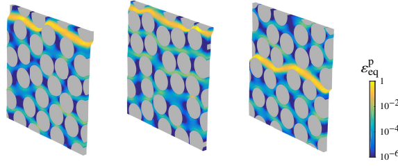
Figure 5: Final equivalent plastic strain distribution from three different micromodels under longitudinal shear with 25 fibers.
