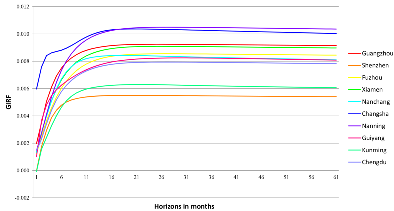
FIGURE 5.4 Generalized impulse responses of a positive unit shock (one standard error) to Changsha house prices
