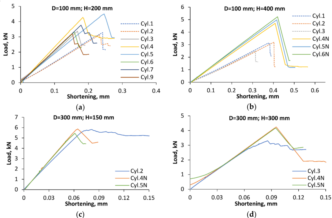
Figure 5. Load–shortening diagrams of cylinders with dimensions: (a) D = 100 mm and H = 200 mm; (b) D = 100 mm and H = 400 mm; (c) D = 300 mm and H = 150; (d) D = 300 mm and H = 300. Results of tests employing a hemispherical joint are plotted by dashed lines, for parallel plates—by solid lines.
