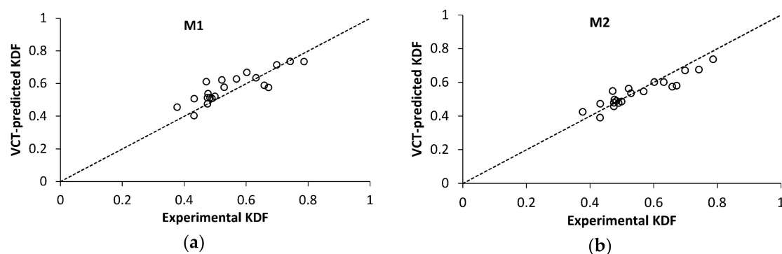
Figure 11. VCT-predicted knock-down factor, using maximum load in vibration tests P/P_b \geq 0.87 , as a function of the experimental KDF for VCT method: (a) M1; (b) M2.
