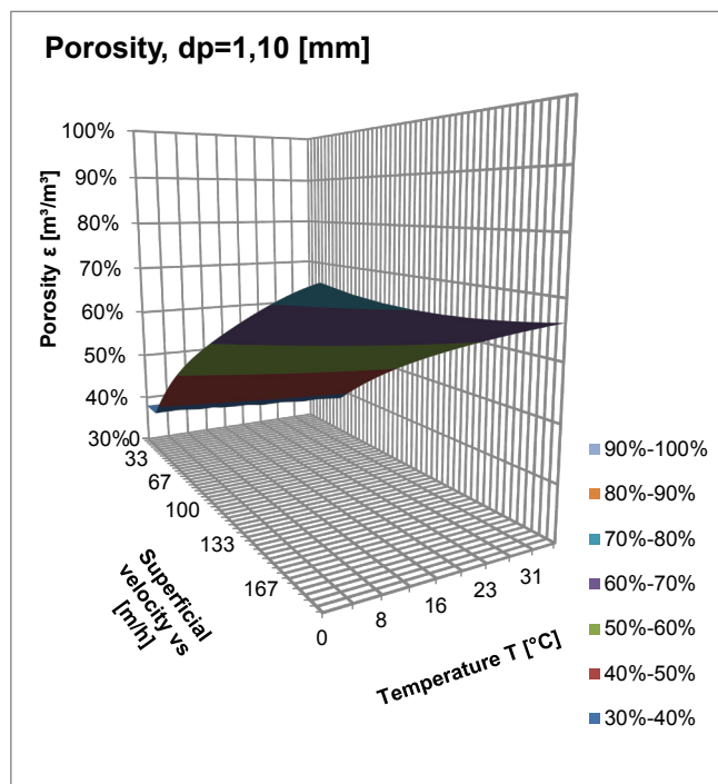
Figure 2: Example of the predicted porosity as a function of superficial water velocity and water temperature.
