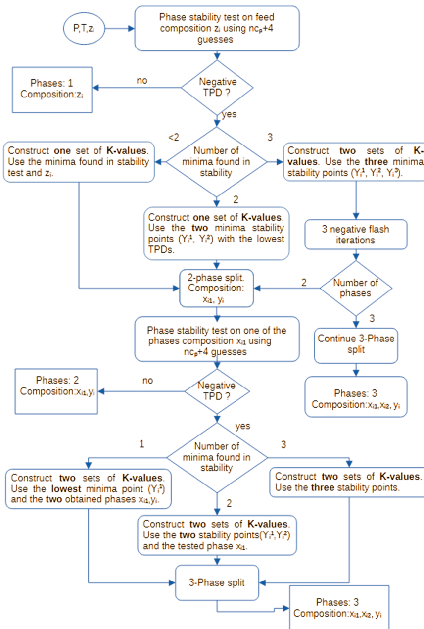
Fig. A3. Flowchart of the IMI method.
