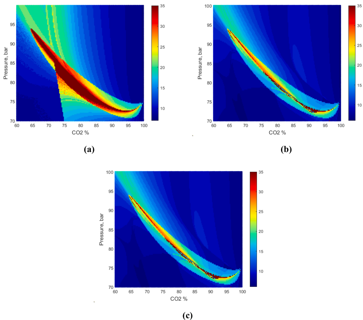
Fig. 11. Total number of multiphase split iterations for Maljamar reservoir mixture results at T = 305.35 K: (a) conventional; (b) ISI; (c) IML.
