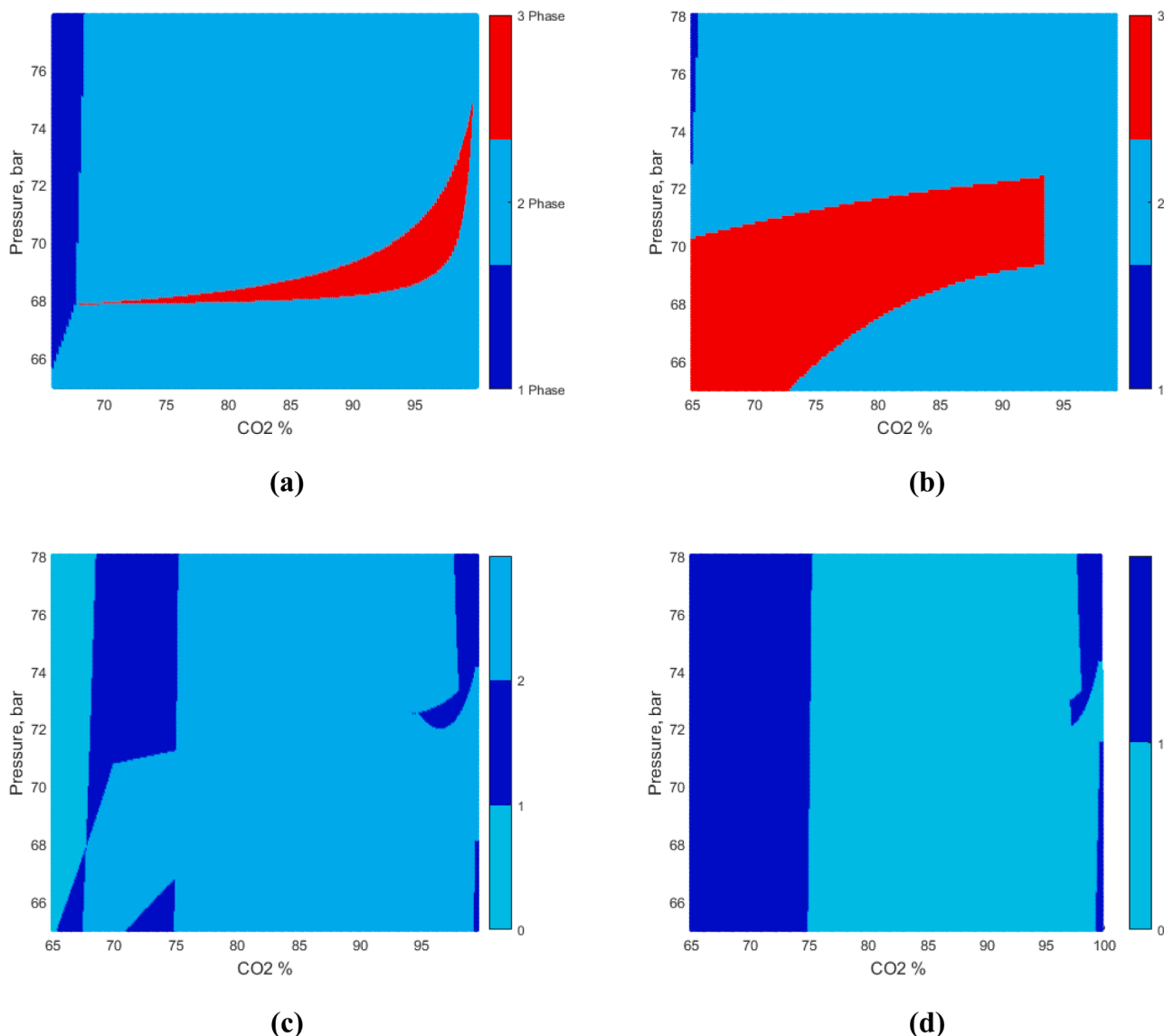
Fig. 13. Maljamar separator mixture results at T = 305.35 K: (a) phase boundaries; (b) total number of minima in one-phase stability; (c) number of minima with negative TPDs in one-phase stability; (d) number of minima with trivial solution in one-phase stability.
