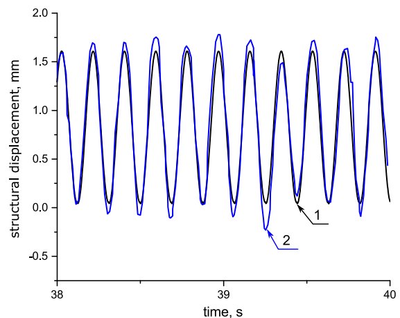
Fig. 6 The dependence of the displacement on time during frequency lock-in at an indentation speed of 0.18 \text{ msec}^{-1} (Curve 1: model results as obtained in this paper; Curve 2: experimental data from [28])
