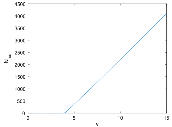
Fig. 8 This plot shows a typical dependence of N_{\text{res}}(v) . Here \kappa = 0.3 , the velocity v lies in the interval [0, 15] and \Omega_n are uniformly distributed in the interval [3, 10] with the step-size 0.07
