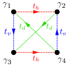
FIG. 4. Four weakly coupled Majorana modes. The coupling amplitude between each pair of Majorana modes is proportional to the strength of the mutual coupling t_\alpha and a phase factor s_{mn} = \pm i . The sign of the phase factor is constrained by the Z_2 gauge symmetry of the magnetic field and is indicated by the arrow: coupling along the arrow direction gives s = i , while coupling opposite to the arrow direction gives s = -i .
