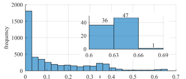
Fig. 13. Histogram of the k values for data set 1.
