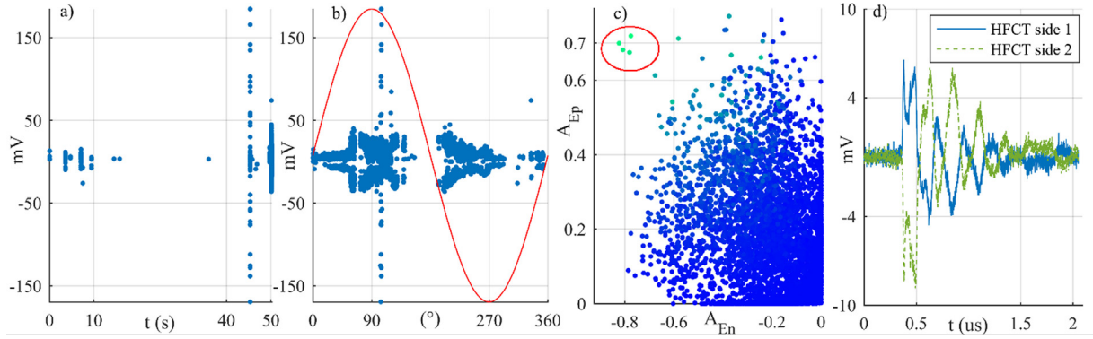
Fig. 16. Application case 1. (a) PD peak voltage in time, (b) PRPD pattern of the whole data set 2, (c) A_{Ep} - A_{En} graph, (d) PD waveforms.
