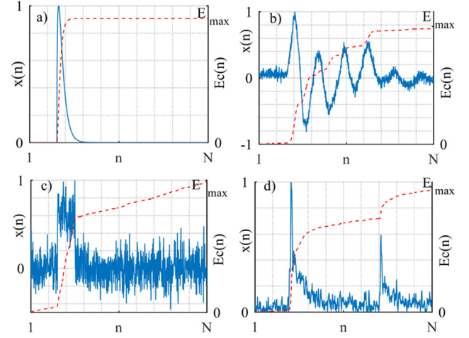
Fig. 1. Examples of the cumulative energy function (dotted line) for different type of signals: (a) fast, unipolar pulse, (b) oscillating pulse, (c) unipolar pulse with low SNR, (d) pulse with a second pulse (disturbance) within the same record window.
