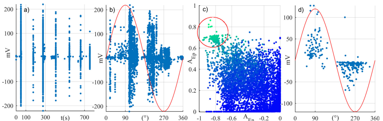
Fig. 17. Application case 2. (a) PD peak voltage in time, (b) PRPD pattern of the whole data set 3, (c) A_{Ep} - A_{En} graph, (d) PRPD pattern of clustered data.
