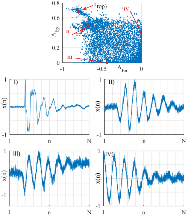
Fig. 9. Waveforms of the signals corresponding to labels in the normalized graph on top.
