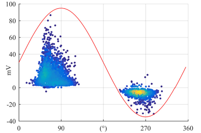
Fig. 18. Example of surface PRPD from the defect under 46kVAC test voltage.
