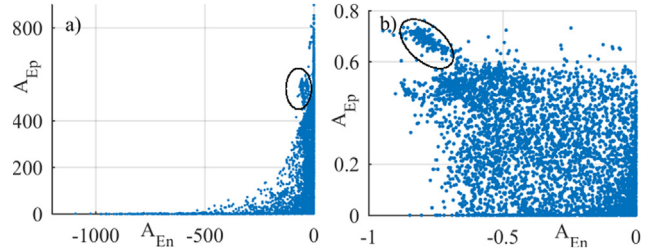
Fig. 8. A_{En} and A_{Ep} graph for data set 1 (a) before normalization, (b) after normalization.
