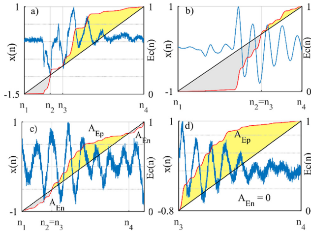
Fig. 6. Examples of signals leading to different relationships between A_{En} and A_{Ep} . (a) A_{Ep} \gg A_{En} , (b) A_{Ep} \ll A_{En} , (c) multiple areas of A_{En} , (d) A_{En} = 0 .
