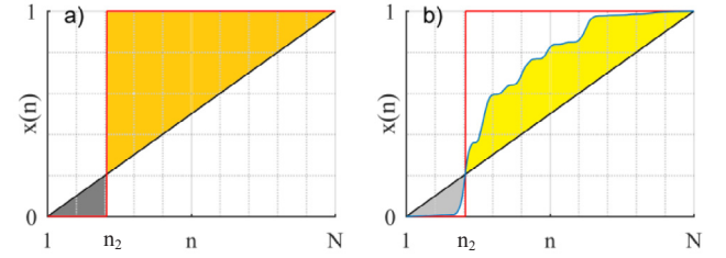
Fig. 7. Comparison of the areas A_{En} and A_{Ep} for (a) Dirac delta pulse and (b) a signal like the one in Fig. 1(b).
