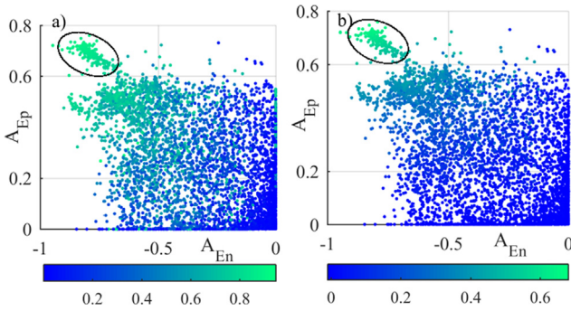
Fig. 14. (a) Color map representing k_1 k_2 k_3 , (b) color map representing k_1 k_2 k_3 A_{Ep} . (For interpretation of the references to colour in this figure legend, the reader is referred to the web version of this article.)
