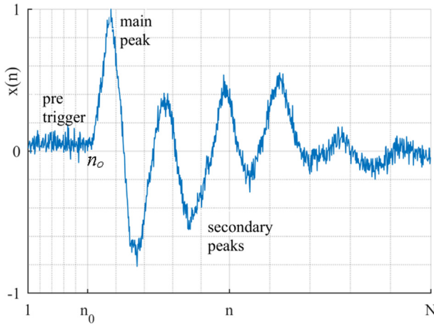
Fig. 2. Definition of the characteristics of a pulse-shaped signal.
