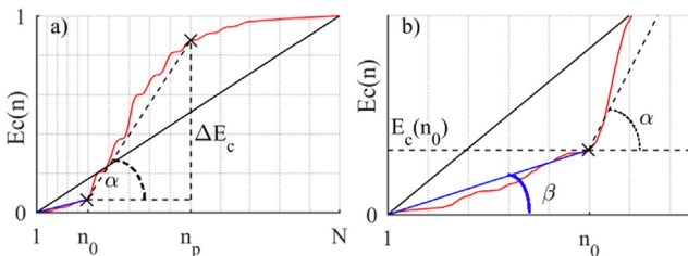
Fig. 10. (a) Metrics in the definition of the shape factor k , (b) zoom-in to illustrate the definition of the angle \beta .
