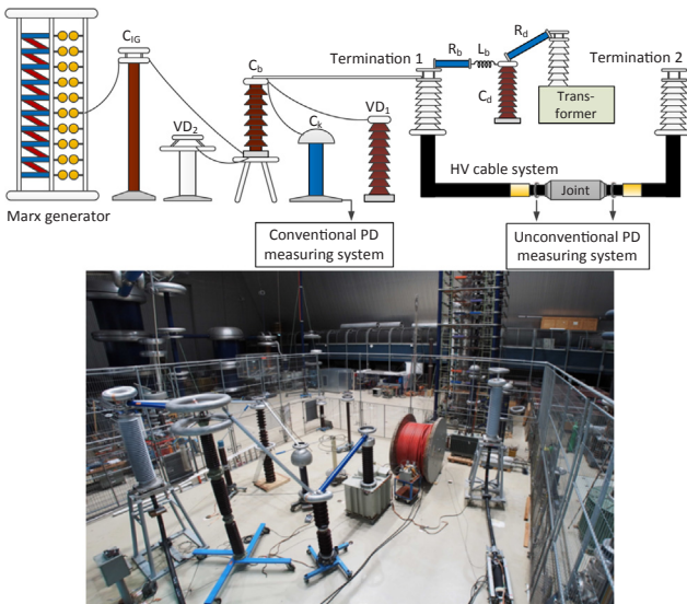
Fig. 15. Superimposed impulse test circuit used for acquiring the data sets 1 and 2. More details can be found in [16].
