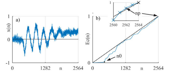
Fig. 12. (a) signal with offset, (b) resulting in a continuous increase of energy.
