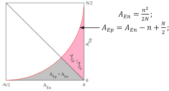
Fig. 5. Geometrical space of A_{En} and A_{Ep} .
