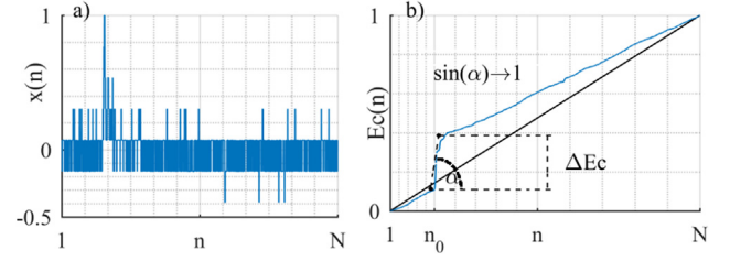
Fig. 11. (a) Signal with low SNR, (b) resulting in a stepped but small increase of energy.
