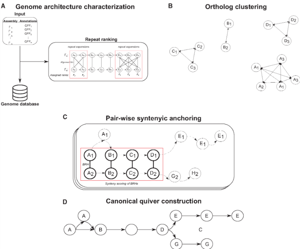
Figure 6.2: Overview of Ptolemy . (A) Ptolemy first creates a database characterizing individual genome architectures for a given list of assemblies and their corresponding gene annotations. In this process, Ptolemy also attempts to identify repeat expansion through self-pairwise gene alignments. (B) Best reciprocal hits (BRHs) are then identified via pairwise gene alignment for every pair of genomes. (C) Syntenic anchors are derived for each BRH by scoring the synteny of the surrounding region of corresponding genes. This is done in a pairwise fashion for every pair of genomes. (D) The syntenic anchors are then used to construct the canonical quiver for all genomes in the database.
