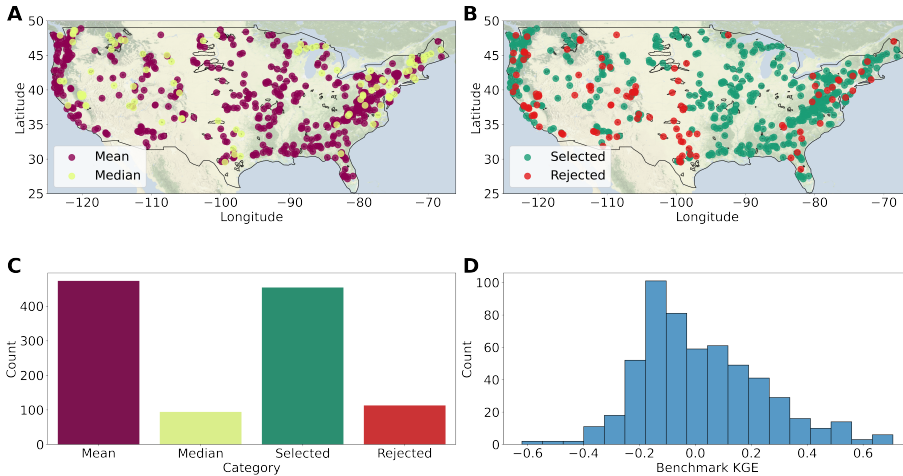
Figure 3.5: Evaluation-period results. (a) The best-performing type of 10-year calendar-day climatology, either mean (purple) or median (yellow). (b) The spatial distribution of accepted (green) and rejected (red) basins based on the benchmark. (c) Overview of the number of basins that are accepted or rejected and the best-performing benchmark type. (d) The KGE 2012 score distribution of the best-performing benchmark type. Basemaps are made with Natural Earth.
