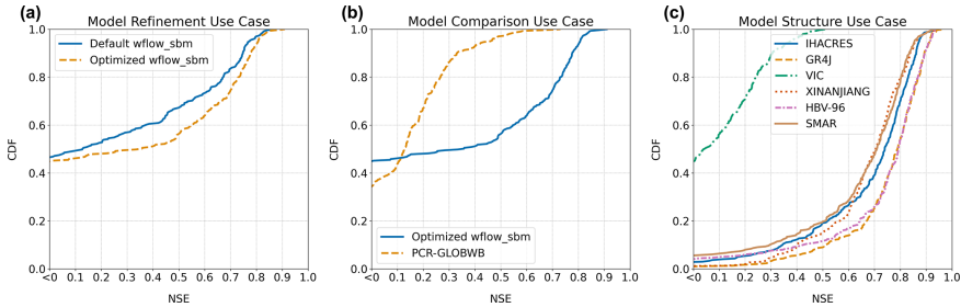
Figure 5.9: Cumulative distribution function plots of the Nash–Sutcliffe efficiency (NSE), derived from discharge estimates and observations at 299 catchment outlets. (a) The model refinement use case, optimizing the wflow_sbm hydrological model with a single parameter. (b) The model comparison use case, comparing the optimized wflow_sbm and PCR-GLOBWB hydrological models. (c) The model structure use case, showing results from 6 conceptual hydrological models.
