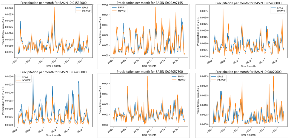
Figure 3.12: ERA5 and MSWEP forcing comparison for six basins in the CAMELS data set. Monthly precipitation values for the evaluation period are shown for ERA5 in blue and MSWEP in orange.
