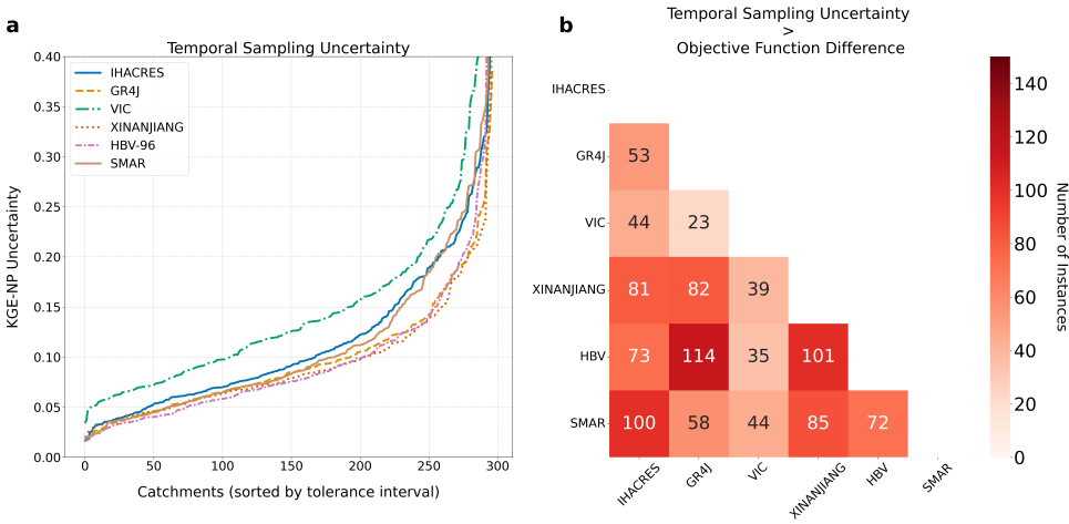
Figure 5.7: (a) Temporal objective function sampling uncertainty based on 6 conceptual hydrological models, expressed as the average tolerance interval of the standard error due to sub-sampling. The sorted values per catchment are shown on the horizontal axis, and the KGE-NP objective function uncertainty is shown on the vertical axis. (b) Heat map of the 6 conceptual hydrological models showing, for each model combination, the number of instances ( n = 299 ) in which the average objective function uncertainty exceeds the objective function differences between model combinations. Low values in white and high values in red indicate the number of instances.
