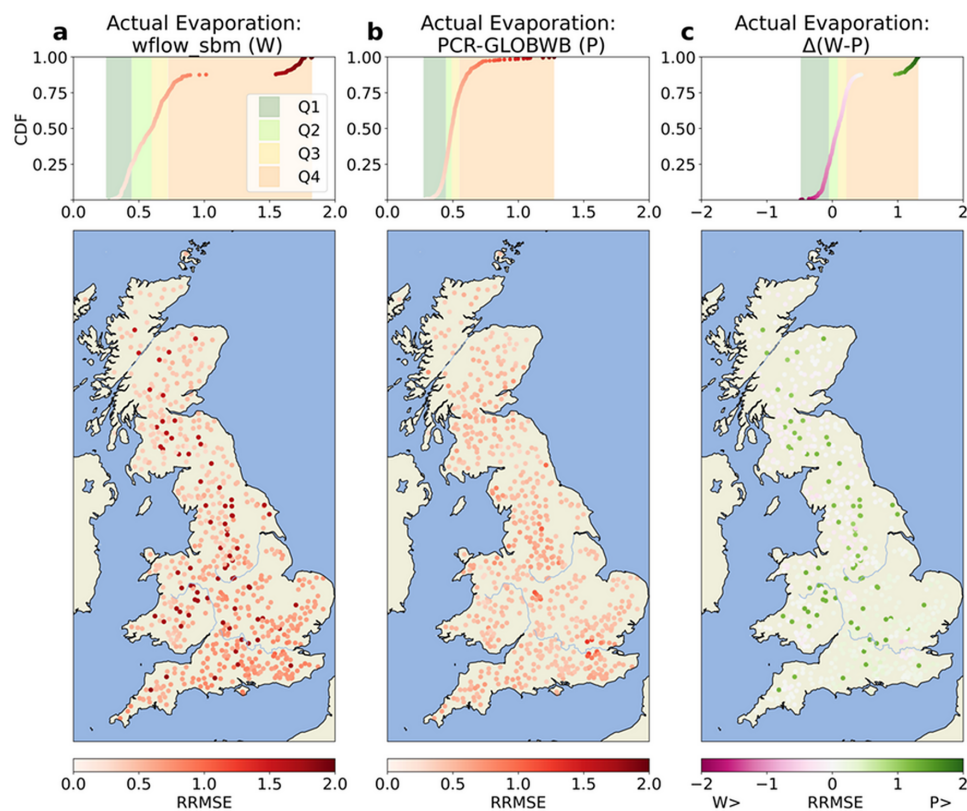
Figure 4.5: Comparison of catchment-averaged, actual evaporation-based model performance using the 8-day-average RRMSE metric. The top panels show the cumulative distribution functions and distribution quantiles (Q1–Q4), and the bottom panels show the spatial distributions of model performance. (a) Wflow_sbm performance, with low RRMSE values in white and high values in red. (b) PCR-GLOBWB performance. (c) Performance difference between the two models, \Delta(W-P) , with better wflow_sbm performance in purple and better PCR-GLOBWB performance in green. Note that this color order is the reverse of that in Figure 4.3.
