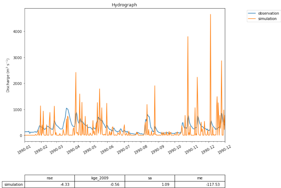
Figure 2.5: A first hydrograph generated with eWaterCycle. This shows the output of the MARRMoT M01 model (a single bucket representing the entire Merrimack basin) when ERA5 is used as forcing data. While the over-simplification of representing the entire basin with a single bucket is clear, the timing of high-flow periods is still rather well represented. This figure is generated using the hydrograph() function, a standard method within the eWaterCycle package. In addition to plotting a hydrograph of the provided time series, it calculates often used metrics like the Nash–Sutcliffe efficiency and the Kling–Gupta efficiency. This example is used as a first ‘hello world’ use case illustrating with a simple model how the eWaterCycle platform supports standard workflows often used in computational hydrological research.
