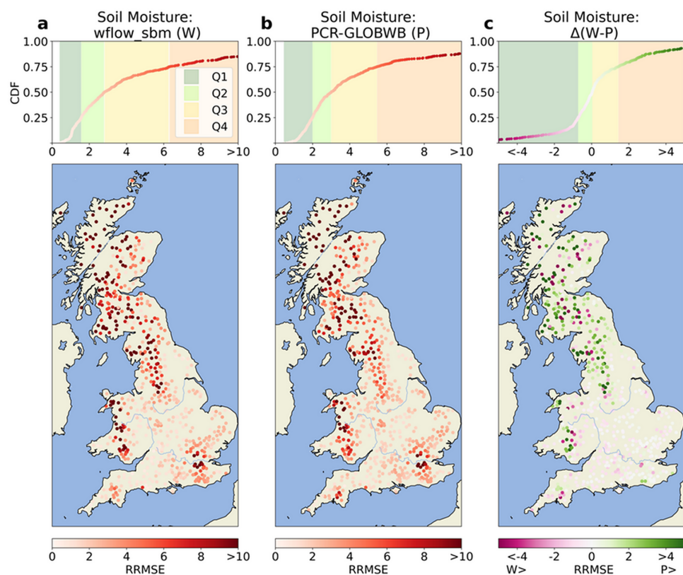
Figure 4.7: Comparison of catchment-averaged, soil moisture-based model performance using the daily-average RRMSE metric. The top panels show the cumulative distribution functions and distribution quantiles (Q1–Q4), and the bottom panels show the spatial distributions of model performance. (a) Wflow_sbm performance, with low RRMSE values in white and high values in red. (b) PCR-GLOBWB performance. (c) Performance difference between the two models, \Delta(W-P) , with better wflow_sbm performance in purple and better PCR-GLOBWB performance in green. Note that this color order is the reverse of that in Figure 4.3.
