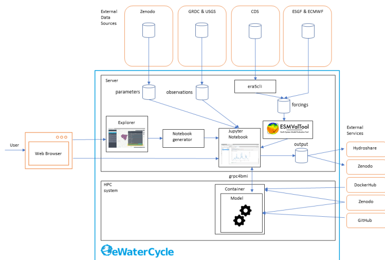
Figure 2.2: The technological design of the eWaterCycle platform, including external services. This overview shows the different components that are, on purpose, built as separate entities to facilitate re-use in other projects. The different components of this technical overview are discussed in detail in the main text of this publication.
