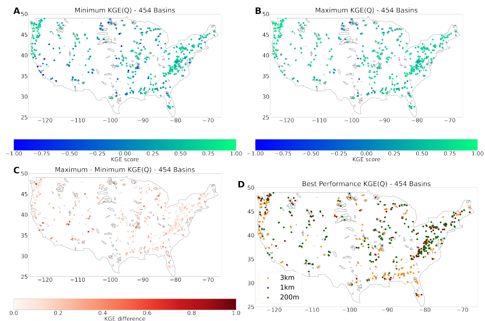
Figure 3.10: Evaluation-period results. (a) Minimum KGE score of the model instances. (b) Maximum KGE score of the model instances. (c) The difference between the minimum and maximum KGE scores. (d) Best-performing model instance based on KGE score for the evaluation period with 3 km in orange, 1 km in red, and 200 m in green.
