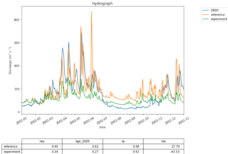
Figure 2.13: This graph shows the effect of intervening in the state of the PCR-GLOBWB 2.0 model. The calculated discharge for the Merrimack basin from two model runs is shown: one reference run in which the model is run without intervention and one experiment in which the model state is changed at every time step to incorporate evaporation observation data from FLUXNET (Pastorello et al., 2020). The calculated discharge for both model runs is compared to GRDC observations of discharge.
