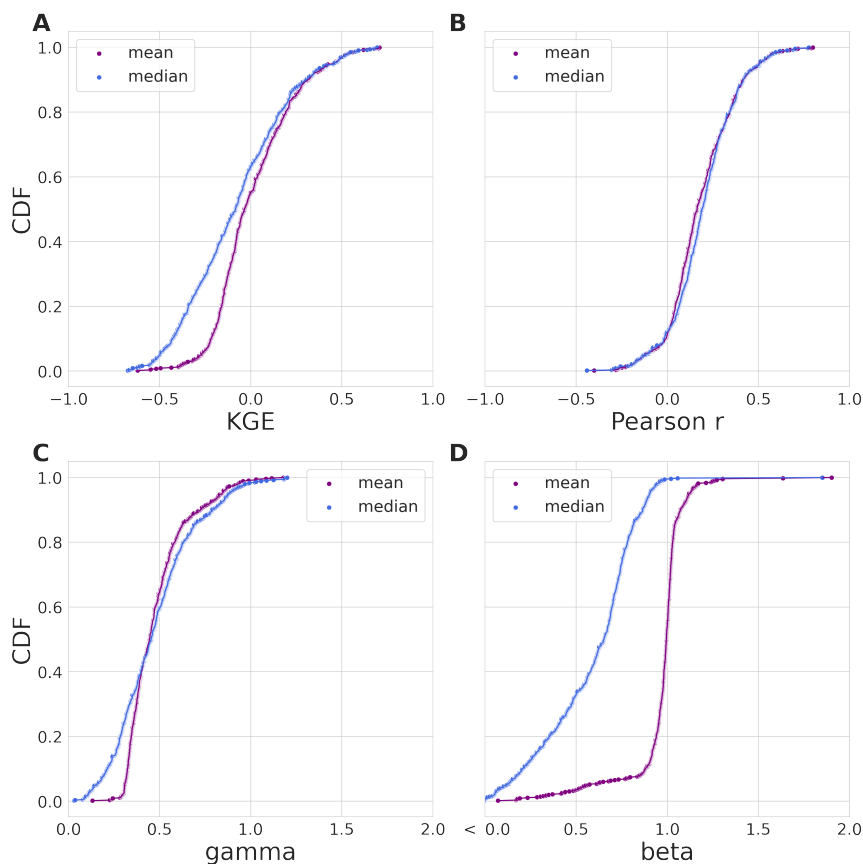
Figure 3.6: Evaluation-period results. The CDFs of the modified KGE score and its 3 individual components for the statistical benchmarks during the evaluation period. The mean statistical benchmark is shown in purple and the median benchmark in blue. (a) The CDF of the modified KGE score. (b) The CDF of the Pearson r correlation KGE component. (c) The CDF of the Gamma (variability ratio) KGE component. (d) The CDF of the Beta (bias ratio) KGE component.
