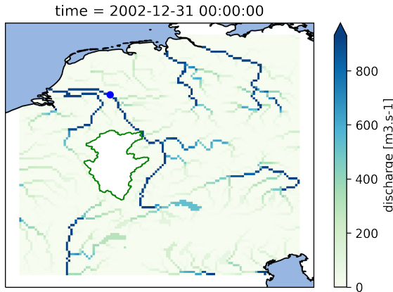
Figure 2.9: Calculated discharge in the Rhine basin at the end of the model run using the PCR-GLOBWB 2.0 model for the Rhine coupled with the simplest one-bucket model from the MARRMoT suite of models for the Moselle subcatchment. The Moselle subcatchment has been cut out of the PCR-GLOBWB 2.0 model (by altering its 'landmask' setting). MARRMoT calculates the discharge for the Moselle and, at each time step, this is added to the 'channel storage' variable of PCR-GLOBWB 2.0 at the location where the Moselle flows into the Rhine (at Koblenz). The blue dot on the map indicates the location of the observation station at Lobith, which is used for the hydrographs shown in Figure 2.11.
