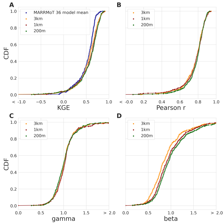
Figure 3.8: Evaluation-period results. The CDFs are based on the modified KGE scores and their 3 individual components for the 454 selected basins. (a) The modified KGE score with the MARRMoT 36-model mean results shown in blue, the 3 km instance in yellow, the 1 km instance in red, and the 200 m instance in green. (b) The Pearson r correlation component. (c) The gamma variability component. (d) The beta bias component.
