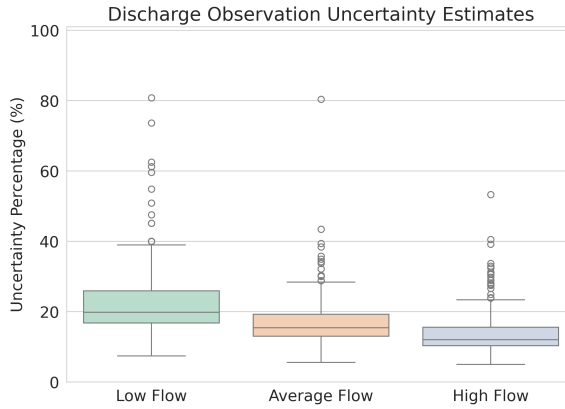
Figure 5.5: Discharge observation uncertainty estimates of 299 catchment outlets based on the work of Coxon et al., 2015 expressed as uncertainty percentages per flow category. (a) the low flow category uncertainty estimates are based on the 5th to 25th flow percentiles. (b) presents the 25th to 75th percentile average flow category. (c) the high flow discharge observation uncertainty estimates of the 75th to 95th flow percentiles are shown.
