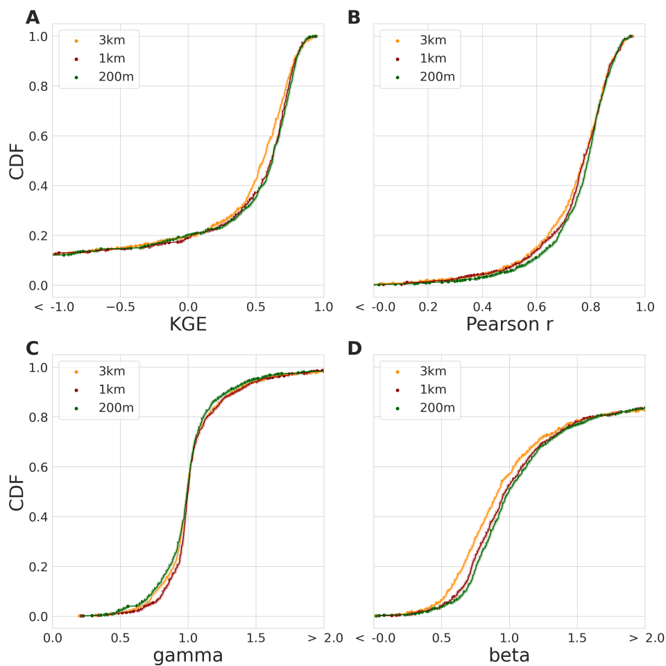
Figure 3.4: Calibration-period results. CDFs of the modified KGE scores and their individual components for the best-performing model runs of the 3 model instances during the calibration period. The 3 km model instance is shown in orange, the 1 km instance in red, and the 200 m instance in green. (a) The CDF of the modified KGE score. (b) The CDF of the Pearson r correlation component. (c) The CDF of the gamma (variability ratio) component. (d) The CDF of the beta (bias ratio) component.
