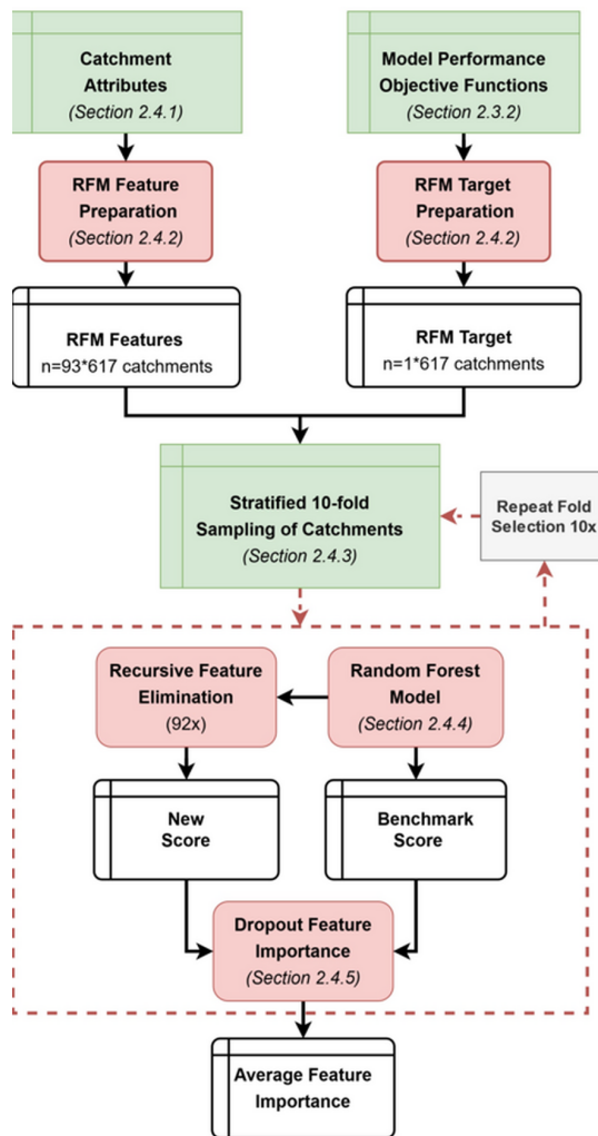
Figure 4.1: Flowchart of the random-forest-model (RFM)-based feature-importance method. (1) A set of model-performance results is selected as the RFM target. (2) Catchment attributes from the CAMELS-GB data set and McMillan et al. (2022) are extracted. (3) The catchment attributes are prepared as RFM features, and the model-performance results as RFM targets. (4) The features and targets for 617 catchments are divided into 10 folds. (5) The RFM is trained using 9 of the 10 folds (approximately 90 % of the catchments) and tested on the remaining fold (approximately 10 %). (6) The benchmark score is calculated using all RFM features. (7) One feature is removed from the complete feature set (93 features), and a new test score is calculated. (8) Dropout feature importance is calculated as the difference between the benchmark score and the new test score. (9) The removed feature is returned to the complete feature set and another feature is removed; this process is repeated until each feature has been removed once. (10) The feature-importance analysis is repeated for all 10 train-test fold combinations before the mean feature importance of each catchment attribute is calculated.
