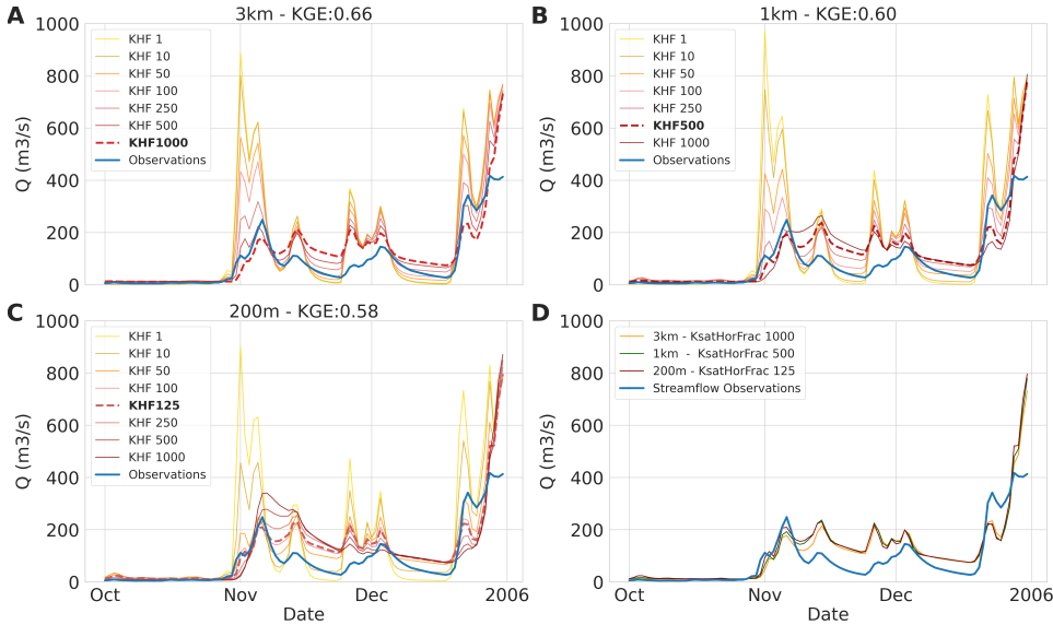
Figure 3.3: Calibration-period results. The calibration interval of the KsatHorFrac parameter (KHF) for the 3 model instances at the basin outlet (ID:14301000) of the final calibration period year. (a) 3 km model instance. (b) 1 km model instance. (c) 200 m model instance. Values range from 1 to 1000 (yellow to red); only a sub-selection is shown. Best-performing calibration values are indicated by a dotted red line and streamflow observations in blue. (d) Best streamflow estimates of the 3 km (orange), 1 km (green), and 200 m (red) model instances.
