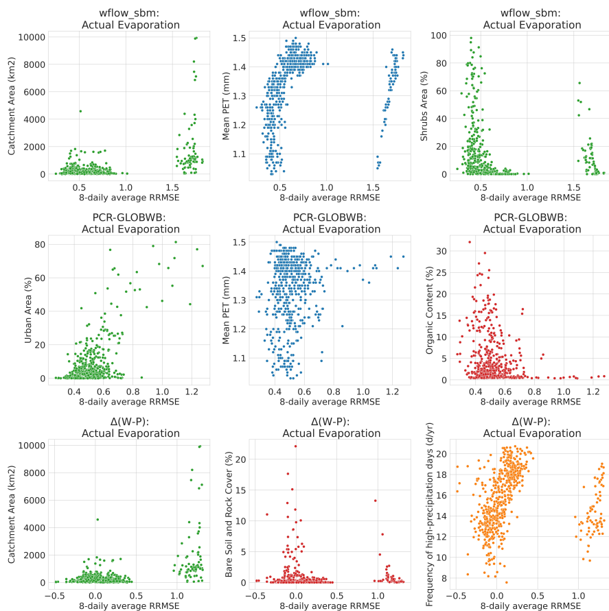
Figure 4.10: Correlations between catchment-attribute values and actual evaporation-based model performance for the three highest-ranking attributes in Table 4.3. Colors indicate attribute classes: land surface (green), hydrology (orange), meteorology (blue), and subsurface (red).
