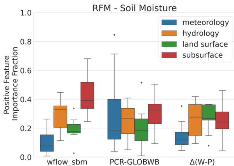
Figure 4.8: Boxplots of the positive feature-importance fraction for each feature class, using catchment attributes as RFM features and soil moisture-based model-performance results as RFM targets. The targets are wflow_sbm (W), PCR-GLOBWB (P), and the performance difference, \Delta(W-P) . Results are grouped into four classes: meteorology (blue), hydrology (orange), land surface (green), and subsurface (red). Each point in a boxplot represents one test fold (Figure 4.2); the variance indicates the degree of spatial variation in the results.
