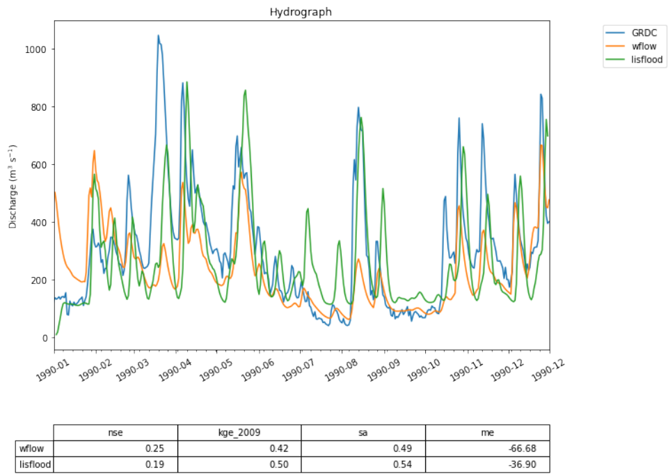
Figure 2.7: Two hydrographs generated by the wflow and the LISFLOOD models compared to GRDC observations for the Merrimack basin. While the code used to run these two models, given in Figure 2.8, is similar to that in the first use case, the models are far more complex and generate better predictions of streamflow.
