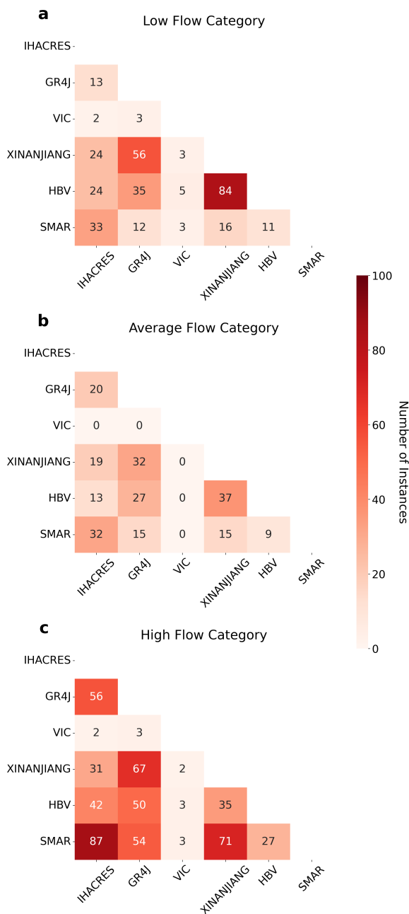
Figure 5.6: Heat map of the 6 conceptual hydrological models showing for each model combination the number of instances ( n=299 ) that discharge observation uncertainty exceeds simulation differences. (a) number of instances for the low flow category, with low values shown in white and high values in red. (b) number of instances for the average flow category. (c) number of instances for the high flow category.
