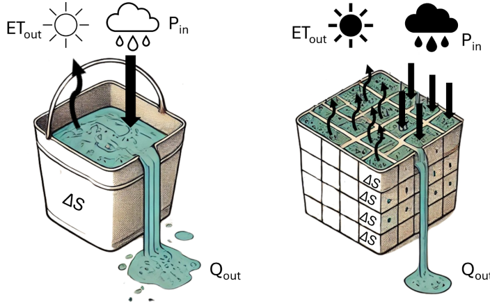
Figure 1.2: Two “leaky bucket” models: a lumped conceptual representation on the left and a physically based distributed representation on the right.
