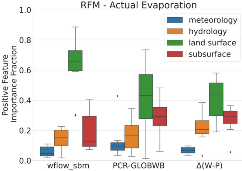
Figure 4.6: Boxplots of the positive feature-importance fraction for each feature class, using catchment attributes as RFM features and actual evaporation-based model-performance results as RFM targets. The targets are wflow_sbm (W), PCR-GLOBWB (P), and the performance difference, \Delta(W-P) . Results are grouped into four classes: meteorology (blue), hydrology (orange), land surface (green), and subsurface (red). Each point in a boxplot represents one test fold (Figure 4.2); the variance indicates the degree of spatial variation in the results.
