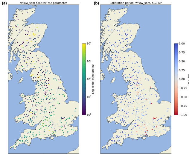
Figure 5.8: (a) Spatial distribution of the best-performing KsatHorFrac calibration parameter of the wflow_sbm model based on additional calibration using discharge observations. (b) Spatial distribution of the KGE-NP objective function based on the calibration period of the wflow_sbm model.
