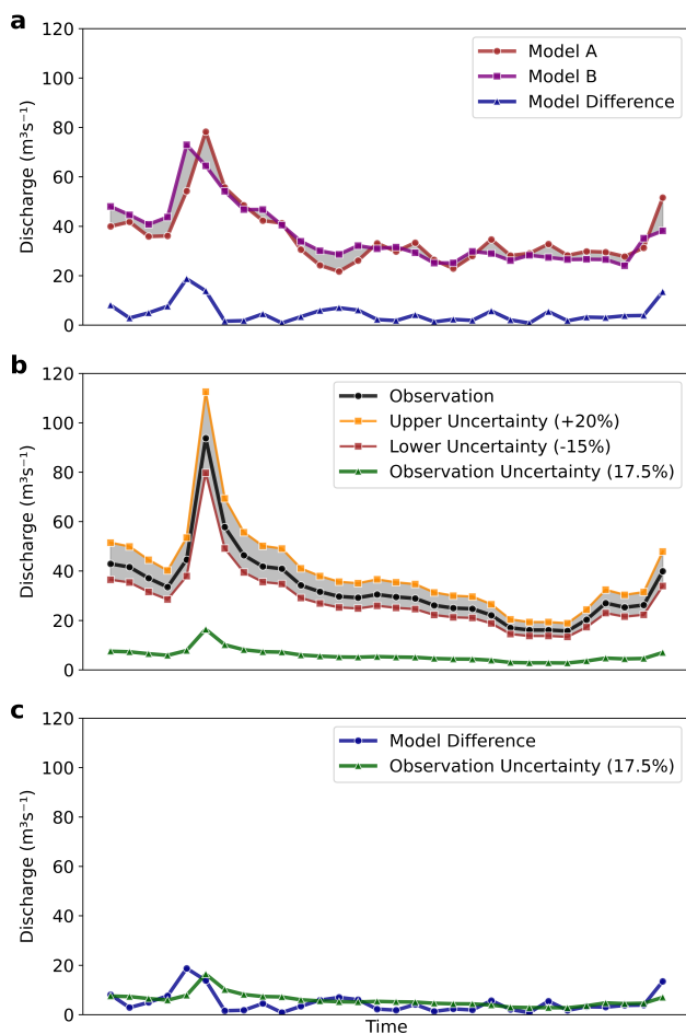
Figure 5.2: Example hydrographs of the discharge observation uncertainty analysis method. (a) Calculation of the absolute difference (blue) between calibrated model simulations (red and purple). (b) Calculation of streamflow observation uncertainty in \text{m}^3 \text{s}^{-1} , shown in green. Orange and dark red lines indicate upper and lower bounds of observation uncertainty percentages that are averaged and multiplied by the observations in black. (c) Resulting time series, with, in blue, the absolute difference between calibrated model simulations and, in green, the averaged discharge observation uncertainty in \text{m}^3 \text{s}^{-1} .
