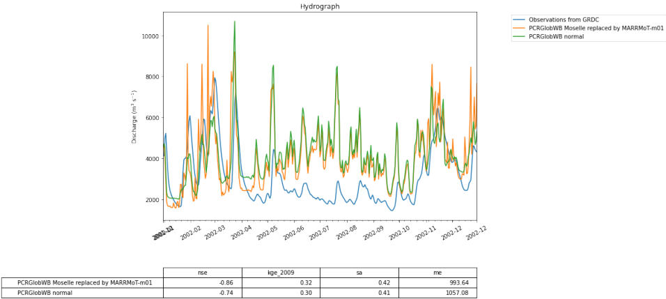
Figure 2.11: The calculated discharge for the Rhine basin from PCR-GLOBWB 2.0 when run normally (i.e., the reference) and when coupled with MARRMoT for the Moselle subcatchment. The calculated discharge is compared to GRDC observations of discharge.
