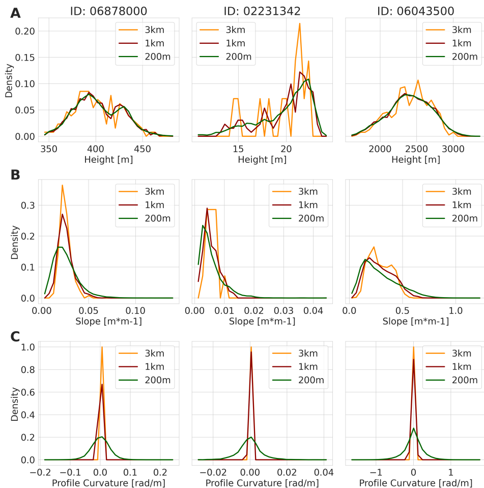
Figure 3.11: 3 example basins representing poor streamflow performance (ID:06878000), moderate performance (ID:02231342), and good performance (ID:06043500). (a) PDFs of height distributions for the 3 km (orange), 1 km (red), and 200 m (green) model instances. (b) PDFs of the slope distributions of the model instances per basin. (c) PDFs of profile-curvature distributions of the model instances per basin. Values equal to 0 indicate linear slope geometry, values smaller than 0 indicate concave slope geometry, and values larger than 0 indicate convex slope geometry.
