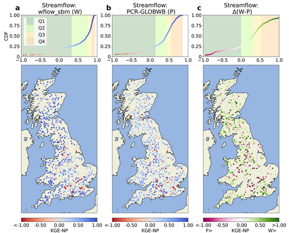
Figure 4.3: Comparison of streamflow-based model performance using the daily KGE-NP metric at the catchment outlet. The top panels show the cumulative distribution functions and distribution quantiles (Q1–Q4), and the bottom panels show the spatial distributions of model performance. (a) Wflow_sbm performance, with low KGE-NP values in red and high values in blue. (b) PCR-GLOBWB performance. (c) Performance difference between the two models, \Delta(W-P) , with better PCR-GLOBWB performance in purple and better wflow_sbm performance in green.
