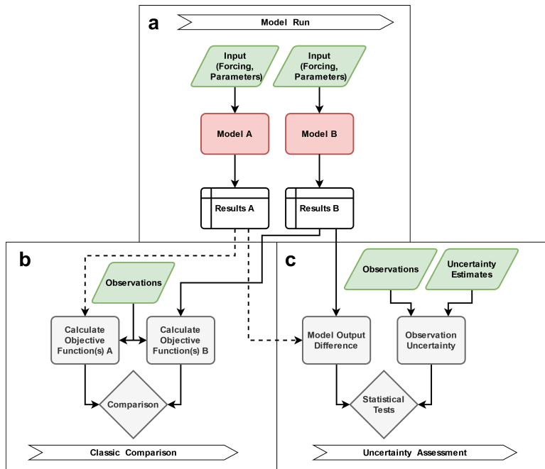
Figure 5.1: Graphical workflow of model experiments and analyses. The model experiment inputs are shown in green, the models in red, and the analysis components in grey. (a) the model runs of two models with inputs and outputs that result in simulation time series. (b) the conventional model comparison that compares objective functions based on simulation and observation time series. (c) the workflow of the proposed analysis that compares relative model simulation differences to discharge observation uncertainty estimates.
