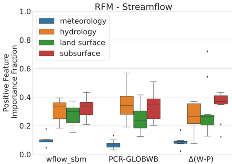
Figure 4.4: Boxplots of the positive feature-importance fraction for each feature class, using catchment attributes as RFM features and streamflow-based model-performance results as RFM targets. The targets are wflow_sbm (W), PCR-GLOBWB (P), and the difference between the two models, \Delta(W-P) . Results are grouped into four attribute classes: meteorology (blue), hydrology (orange), land surface (green), and subsurface (red). Each point in a boxplot represents one test fold (Figure 4.2); the variance indicates the degree of spatial variation in the results.
