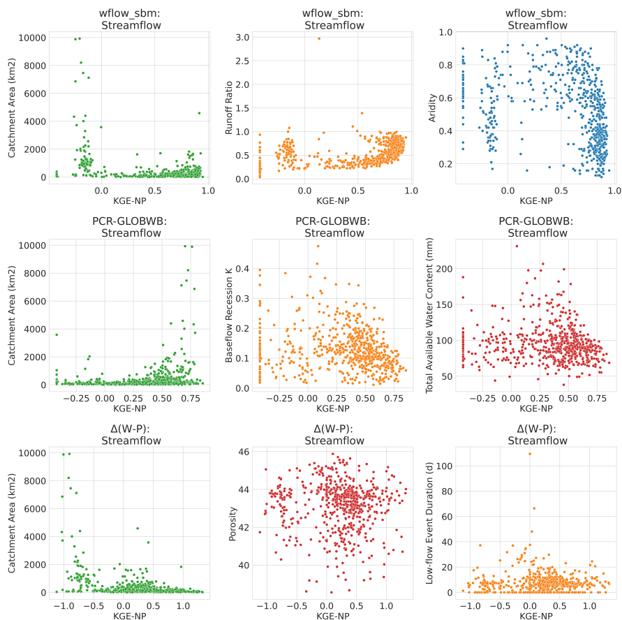
Figure 4.9: Correlations between catchment-attribute values and streamflow-based model performance for the three highest-ranking attributes in Table 4.2. Colors indicate attribute classes: land surface (green), hydrology (orange), meteorology (blue), and subsurface (red).
