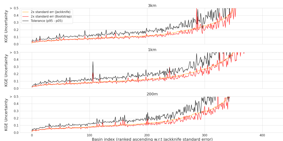
Figure 3.9: Evaluation-period results. The bootstrap and jackknife-after-bootstrap results of the sampling uncertainty of the KGE score. The 2\times standard error of the jackknife method is shown in orange, the 2\times standard error of the bootstrap method in red, and the tolerance interval obtained by subtracting the 5th percentile from the 95th percentile is shown in black. The horizontal axis shows the basin index ranked by the jackknife standard error and the vertical axis shows the modified KGE score sampling uncertainty. (a) 3 km model instance. (b) 1 km model instance. (c) 200 m model instance.
