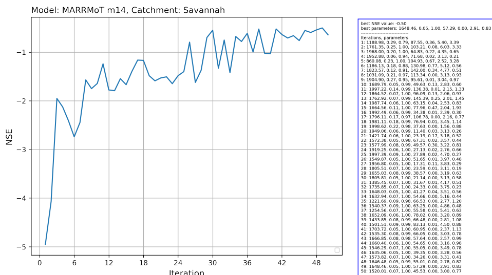
Figure 2.15: Output of the running the Covariance Matrix Adaptation Evolution Strategy (CMA-ES) calibration scheme from the CMA-ES/pycma software package on the MARRMoT m14 model (an implementation of TOPMODEL) for the Savannah basin.
