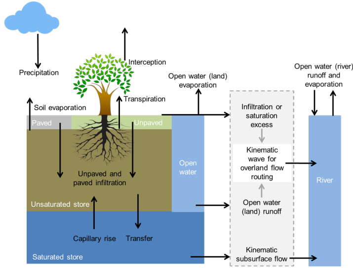
Figure 3.2: Overview of the different processes and fluxes in the wflow_sbm model (Schellekens et al., 2020b).
