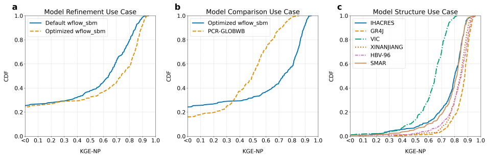
Figure 5.3: Cumulative distribution function (CDF) plots of the Kling-Gupta Efficiency non-parametric (KGE-NP) objective function, derived from discharge estimates and observations at 299 catchment outlets. (a) shows the CDF for the model refinement use case, optimizing the wflow_sbm hydrological model with a single parameter. (b) shows the CDF for the model comparison use case, comparing the optimized wflow_sbm and PCR-GLOBWB hydrological models. (c) demonstrates the CDF for the model structure use case, showcasing results from 6 conceptual hydrological models.
