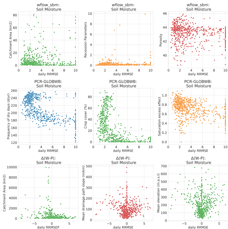
Figure 4.11: Correlations between catchment-attribute values and soil moisture-based model performance for the three highest-ranking attributes in Table 4.4. Colors indicate attribute classes: land surface (green), hydrology (orange), meteorology (blue), and subsurface (red).
