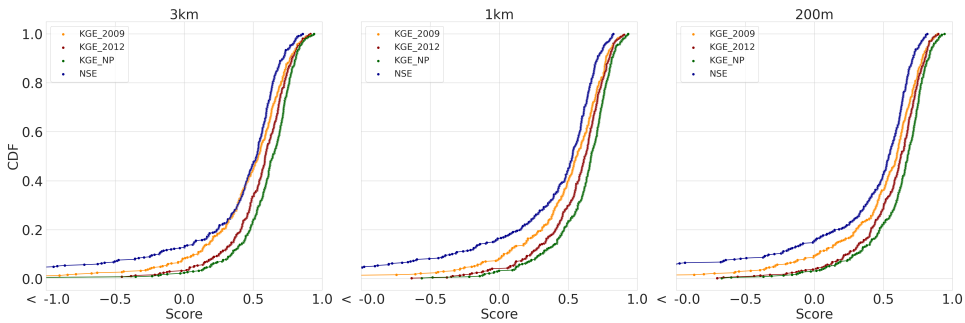
Figure 3.13: Evaluation-period cumulative distribution functions of multiple objective functions for the three model instances, with KGE 2009 in orange, KGE 2012 in red, non-parametric KGE in green, and NSE in blue.
