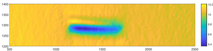
Figure 7: Wind turbine wake at the hub height, in the horizontal plane, at t = 90 s.
