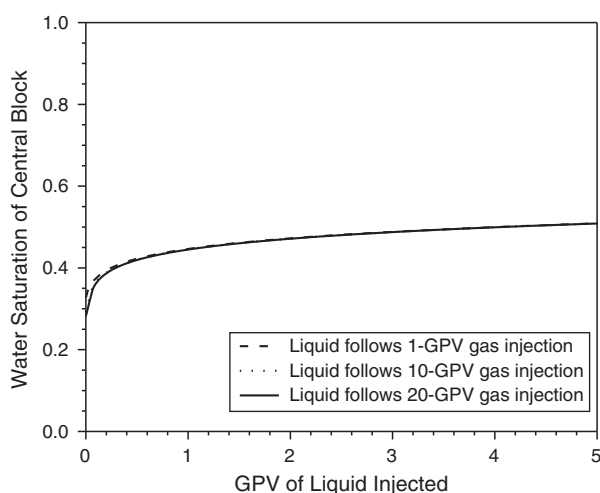
Fig. 14—Water saturation in the gridblock during liquid injection following various periods of gas injection. The curves nearly overlaid each other.
