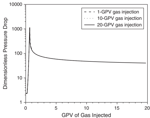
Fig. 11—Dimensionless pressure drop during gas injection, calculated with the Peaceman equation. The dotted, dashed, and solid lines overlaid each other.
