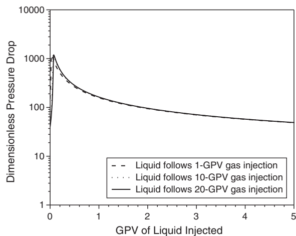
Fig. 13—Dimensionless pressure drop during liquid injection following various periods of gas injection, calculated with the Peaceman equation. The curves nearly overlaid each other.
