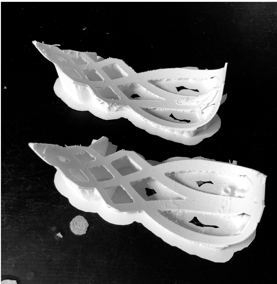
Fig. 59: 3D Printed Petals The selected curved-ribbon petals 3D printed from PLA filament, providing very complicated to separate from the 'tree' support structure.
