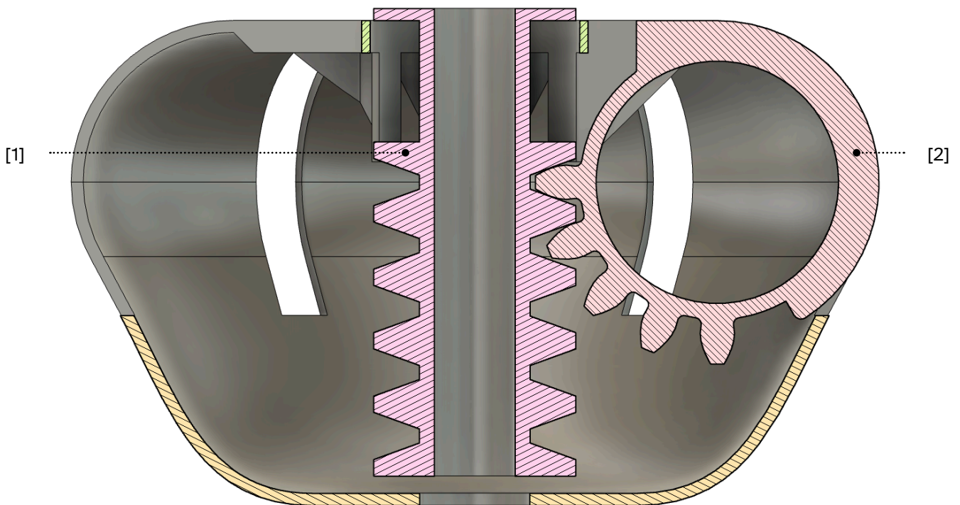
Fig. 47: Rack and Pinion Gear System, Y-Z Cross Section Cylindrical rack gear [1] connected to 1 of 6 total pinion gears [2].
