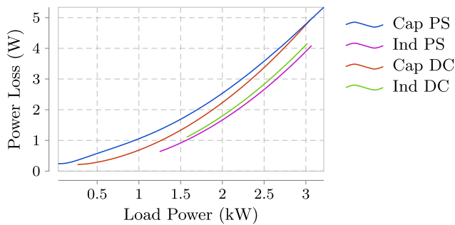
FIGURE 11. Switch conduction losses for all the modes.
