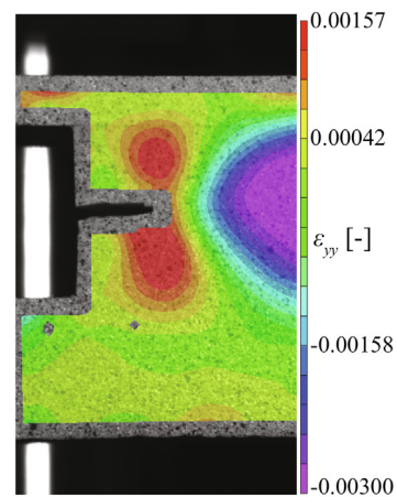
(c) Steel-GFRP bonded joint.
