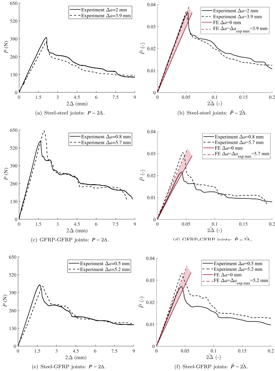
Fig. 6. Experimental load vs. displacement curves: raw ( P - 2\Delta ) and normalized results ( \bar{P} - 2\bar{\Delta} ).
