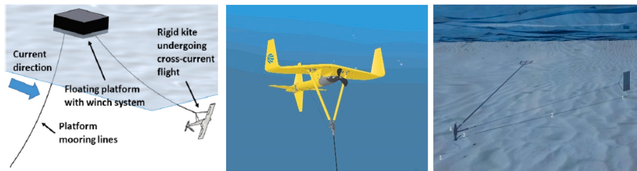
Fig. 30. Major components of an ocean kite system (Cobb et al., 2019a); Minesto Deep Green (Minesto, Ltd, 2021); and SeaCurrent Tidal Kite (SeaCurrent Holding BV, 2021).
