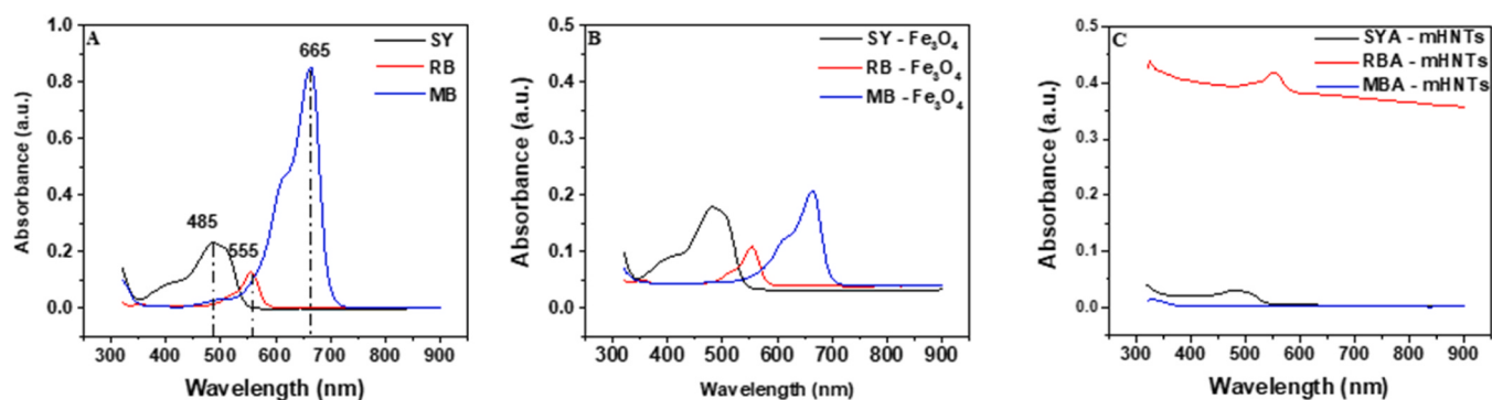
Fig. 9. UV-vis spectroscopy of (A) 0.01 M stock solution of SY, RB and MB dye, (B) Dye solution with \text{Fe}_3\text{O}_4 at pH 7 and (C) dye solution with mHNTs at pH 7.
