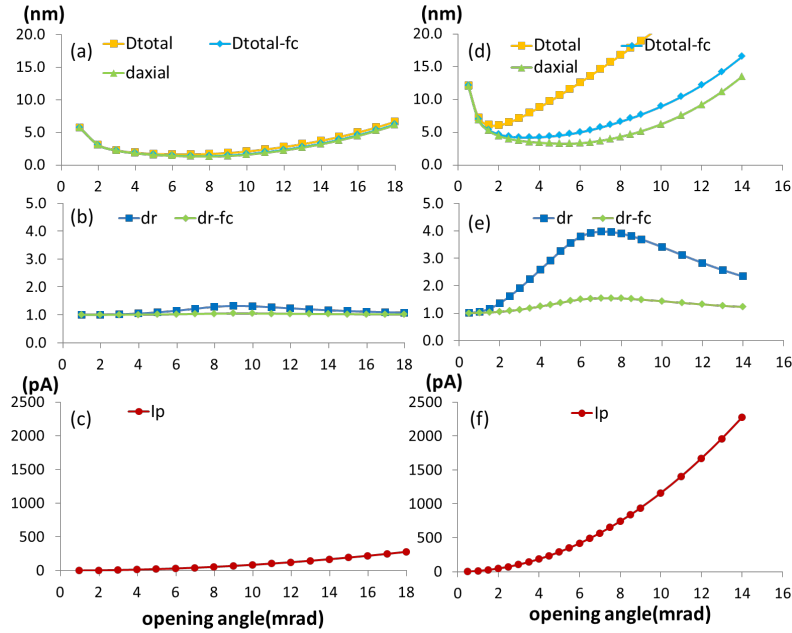
FIG 2. 18 (a), (b) and (c) plots present the result from the combination (ACC3 7000V HR0.3 WD5mm) with 0.5 \mu\text{m} pitch. (d), (e) and (f) plots present the result from the combination (ACC3 7000V HR1.2 WD9mm) with 2.0 \mu\text{m} pitch.
