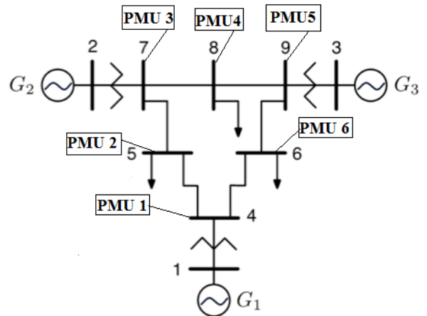
Fig. 2: IEEE 9-bus system with PMUs
