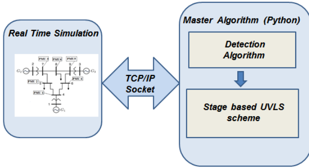
Fig. 1: Diagram of the experimental setup
