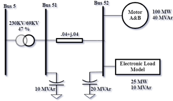
Fig. 3: Composite load model as specified in [15]
