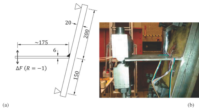
Fig. 9. Specimens of current study for Detail C2a and C2b, steel grade S355: (a) Dimensions (in mm); width = 200 mm; (b) Mounted in set-up.
