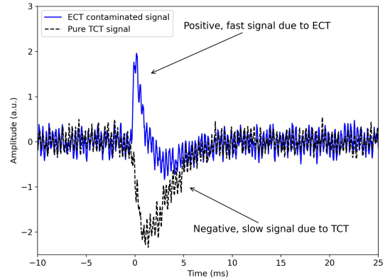
Fig. 3. Example of ECT contaminated signal (blue) and pure TCT signal (black dashed) for the same Victim pixel of Fig. 5.
