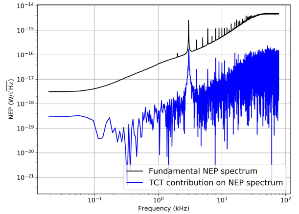
Fig. 7. Example of measured NEP spectrum calculated only with the fundamental noise of the detector (black) and the contribution in quadrature of the thermal crosstalk induced by a nearest neighbor pixel. The resonance at 3 kHz is a consequence of the frequency shift algorithm, used to move the intermodulation distortions at 1.5 kHz and higher harmonics in the demodulated TES response. The excess noise within G(1 + \mathcal{L}_0)/2\pi C \simeq 240 Hz (thermal bandwidth) in the blue curve is a sign of thermal crosstalk.
