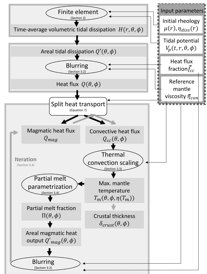
Fig. 1. Flow chart of all modelling steps. Big grey boxes give the three main model steps. The finite element model is described in Section 2 , the blurring, the steady-state scaling, and the partial melt parametrisation and the iteration of the local heat flux fluctuation Q_{\infty}(\theta, \phi) are presented in Section 3 . The dashed box on the right represents the main input parameters, oval boxes give modelling sub-procedures and rectangular boxes display intermediate and final model outputs.
