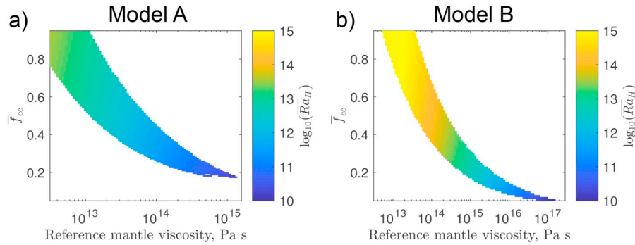
Fig. C.1. Globally averaged Rayleigh-Roberts number as a function of the heat flux fraction \bar{f}_{ce} and the reference mantle viscosity \bar{\eta}_{con} for Model A and Model B.
