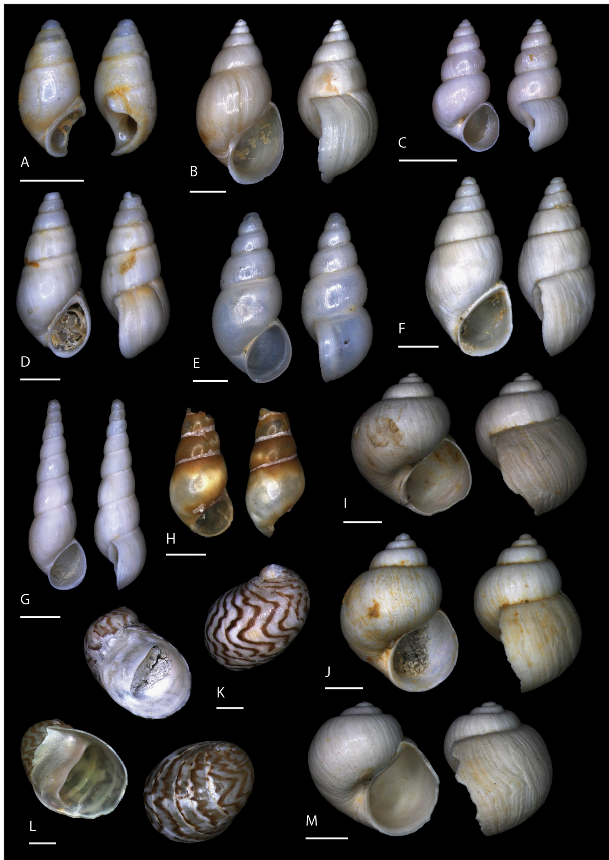
Fig. 7. Late Holocene Novocaspian gastropod species from Turali, with indication of sample and collection number. A Clathrocasia gmelinii : M0203, RGM.1309848 B Clessiniola variabilis : M0204, RGM.1309864 C Ecrobia grimmii : M0202, RGM.1309863 D Laevicaspia sieversii : M0204, RGM.1309849 E Laevicaspia kolesnikoviana : M0221, RGM.1309850 F Laevicaspia conus : M0204, RGM.1309851 G Turricaspiia spica : M0202, RGM.1309858 H Turricaspiia sp. indet. M0222, RGM.962401. I Abeskunus brusinianus : low morph, M0204, RGM.962355 J Abeskunus brusinianus : high morph, M0204, RGM.962355 K Theodoxus pallasi : M0204, RGM.130985, L. Theodoxus pallasi : M0220, RGM.1309862, M Abeskunus exiguus , M0204, RGM.962357. Scale bars 1 mm.
