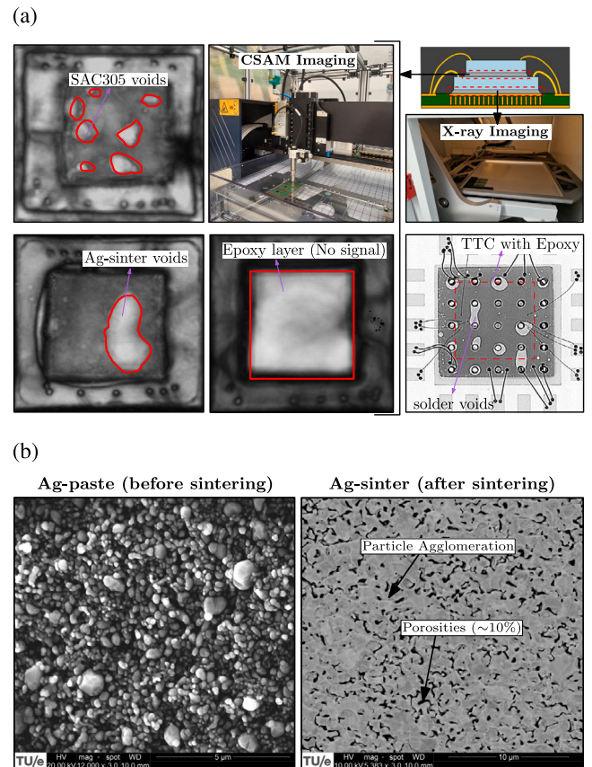
Fig. 3. (a) Inspection of samples using CSAM imaging and X-rays. Voids on the Ag-sintered layer and SAC305 soldered layer were observed. No signal passes through epoxy material due to higher acoustic impedance. X-ray examination indicates voids on the PCB solder layer (below the diode). (b) SEM images of the Ag-paste before sintering (laterally dispensed in a flat plate) and after sintering (vertically cross-sectioned) are shown. Agglomeration of particles with 10% porosities was observed after sintering.
