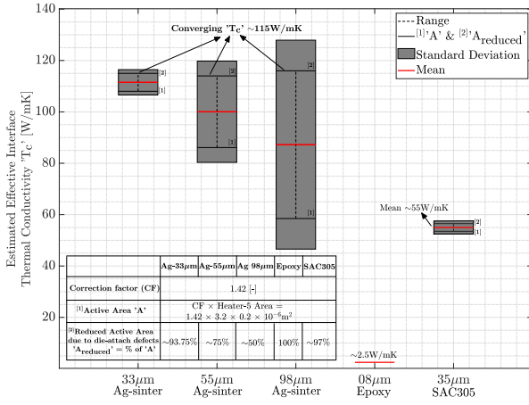
Fig. 10. Standard deviation of effective interface thermal conductivity ' T_c ' estimated based on active area ' A ' and reduced active area ' A_{reduced} ' due to interface defects.
