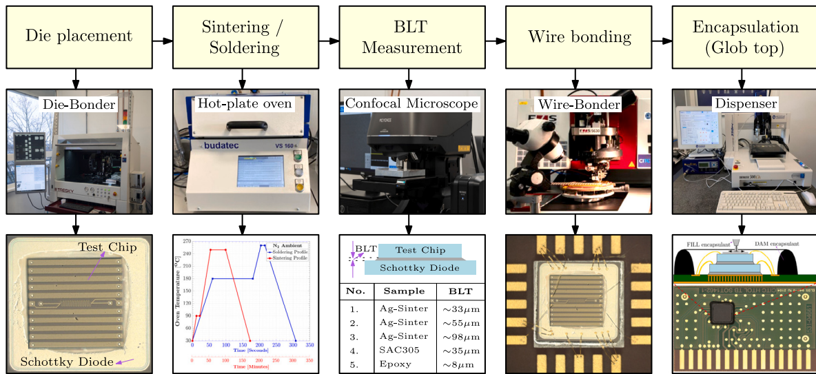
Fig. 2. Illustration of the various package assembly processes involved in sample preparation. The TTC was placed over the diode using a die-bonder and subsequently cured using an industrial hot-plate oven. Upon curing, the interface bond line thickness (BLT) was measured using a confocal laser microscope. The samples were further wire-bonded and encapsulated.
