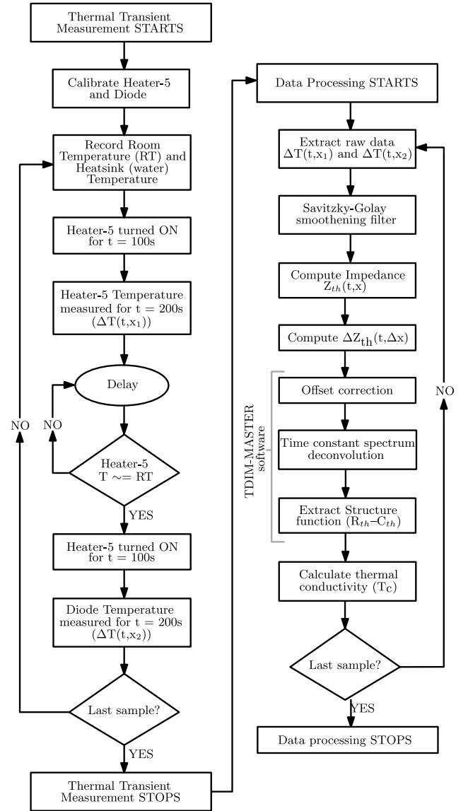
Fig. 5. Flow chart demonstrating the experimental methodology and data processing. All measurements were performed at room temperature ( \sim 25 ^{\circ}\text{C} ). The heat sink temperature was the same as room temperature. The data processing was partly performed using JEDEC TDM-Master software.
