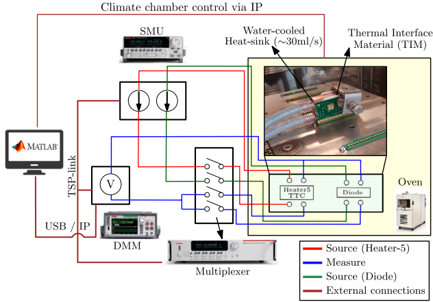
Fig. 4. Schematic illustration of the experimental setup developed for measuring TTC on Diode configuration.
