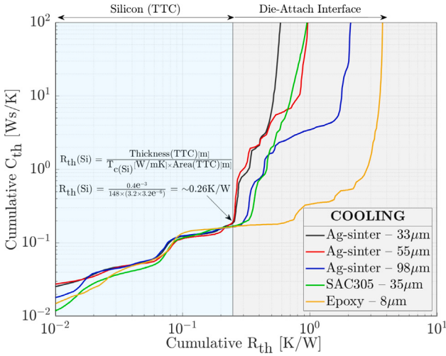
Fig. 8. Cumulative structure function of Ag-sinter ~ 33 \mu\text{m} , ~ 55 \mu\text{m} , ~ 98 \mu\text{m} , SAC305 & Epoxy glue is shown. The Silicon test chip has a resistance of ~0.26 K/W, and the remainder provides the effective thermal resistance of the die-attach interface.
