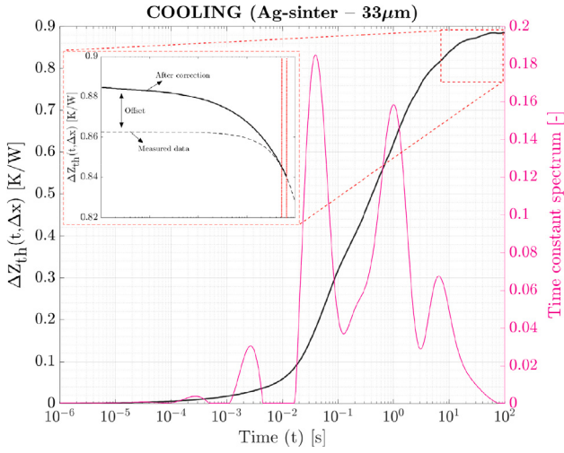
Fig. 7. The offset on heat flux impedance data \Delta Z_{th}(t, \Delta x) was corrected and the time-constant spectrum was determined.
