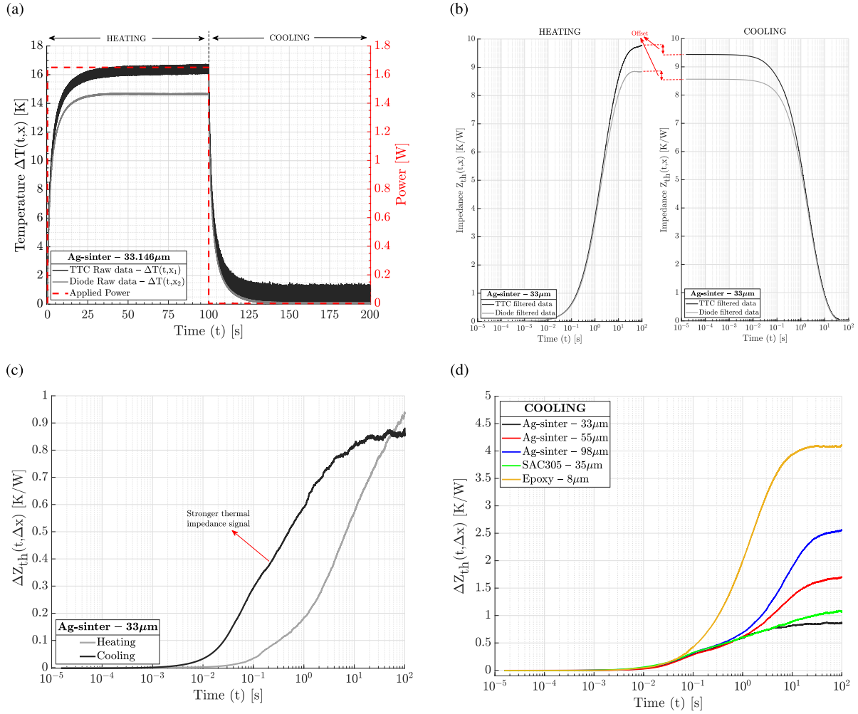
Fig. 6. (a) Raw measurement data of the test chip and the diode is shown along with the applied power input. The test chip has a lower signal-to-noise ratio compared to the diode. (b) Smoothened impedance data is shown on a logarithmic scale, highlighting the offset between heating up and cooling down. (c) The heat flux impedance obtained from the cooling down curve indicates a stronger heat dissipation signal. (d) The heat flux impedance data of all five samples; Ag-sinter \sim 33 \mu\text{m} , \sim 55 \mu\text{m} , and \sim 98 \mu\text{m} ; SAC305 solder paste and non-conductive epoxy glue are shown.
