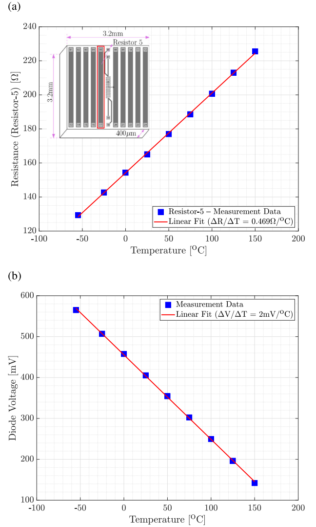
Fig. 1. The resistance sensitivity of Resistor-5 (a) and Schottky diode (b) was evaluated at nine different temperatures, which exhibits a linear temperature dependence.
