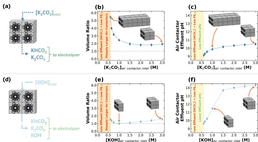
Figure 5. Schemes of (a) K_2CO_3 -fed and (d) KOH-fed air contactors. Air contactor volume ratios of (b) K_2CO_3 -fed and (e) KOH-fed air contactors as functions of the solvent concentration. Air contactor effluent pH as a function of inlet air contactor concentrations of inlet (c) K_2CO_3 and (f) KOH solvents. Note that the drawings of the air contactors indicate the size with respect to the 1 M KOH contactor. For instance, the first point in (b) from the left (0.60 M K_2CO_3 solvent) corresponds to 5.5 times the size of a contactor operating with 1 M KOH solvent, considering the same capture rate of 646 t- CO_2 per year. In all of these cases, the capture fraction was approximately 78%.
