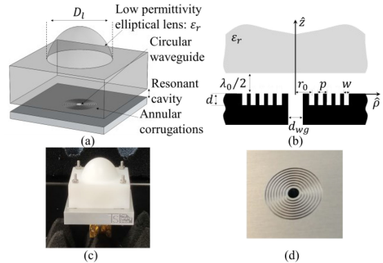
Fig. 1. (a) Geometry of the proposed LW lens antenna. (b) Dimensions of the feed stratification consisting of a circular waveguide, corrugated ground plane, air cavity, and semi-infinite medium. Photographs of (c) the assembled prototype and of (d) the circular waveguide and annular corrugations.
