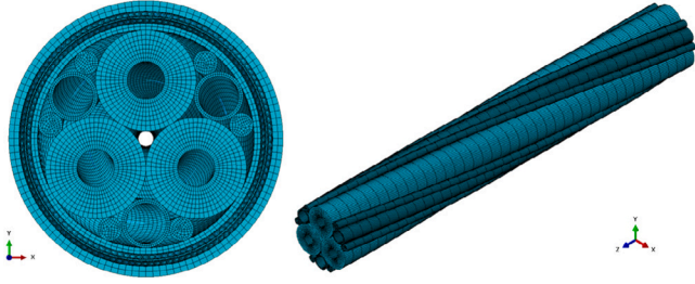
Fig. 17. Mesh of the three-core SPC by using beam &amp; surface helical wires.
