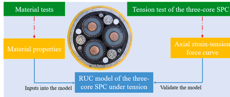
Fig. 7. The calibration and validation flow chart.
