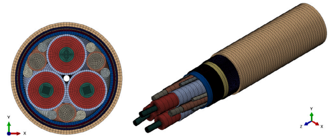
Fig. 15. The RUC model of the three-core SPC.
