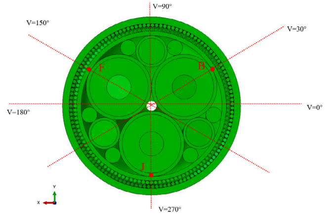
Fig. 24. Illustration of the nodes in the middle cross-section of the three-core SPC.
