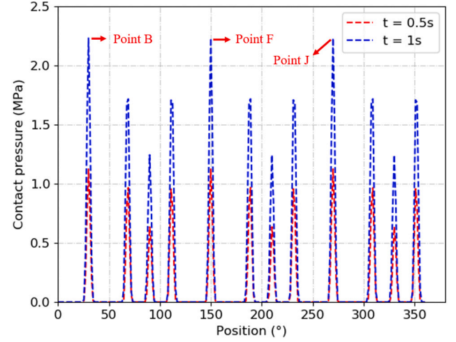
Fig. 23. Contact pressure of the inner sheath under tension.
