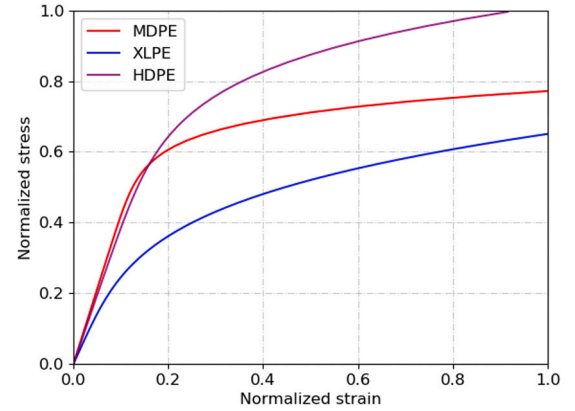
Fig. 12. Normalized strain vs. stress curves for MDPE, XLPE &amp; HDPE.
