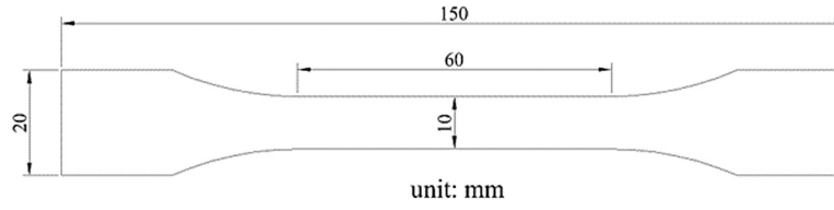
Fig. 9. The detailed dimensions of MDPE &amp; XLPE.
