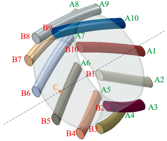
Fig. 4. Nodes involved in periodicity conditions on the helical wire layer.
