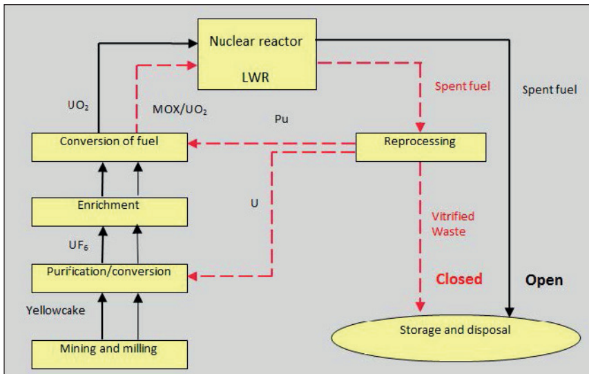
Figure 22: two methods for nuclear power production
