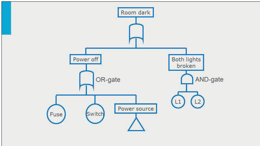
Figure 35: Fault Tree Analysis
