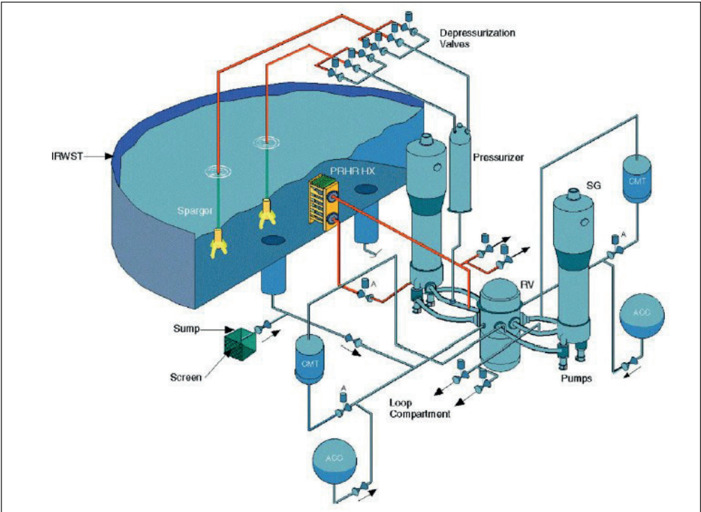
Figure 26: passive core cooling system of the AP1000
