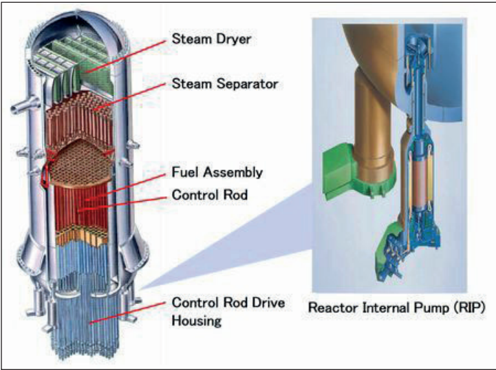
Figure 25: reactor vessel of an ABWR
