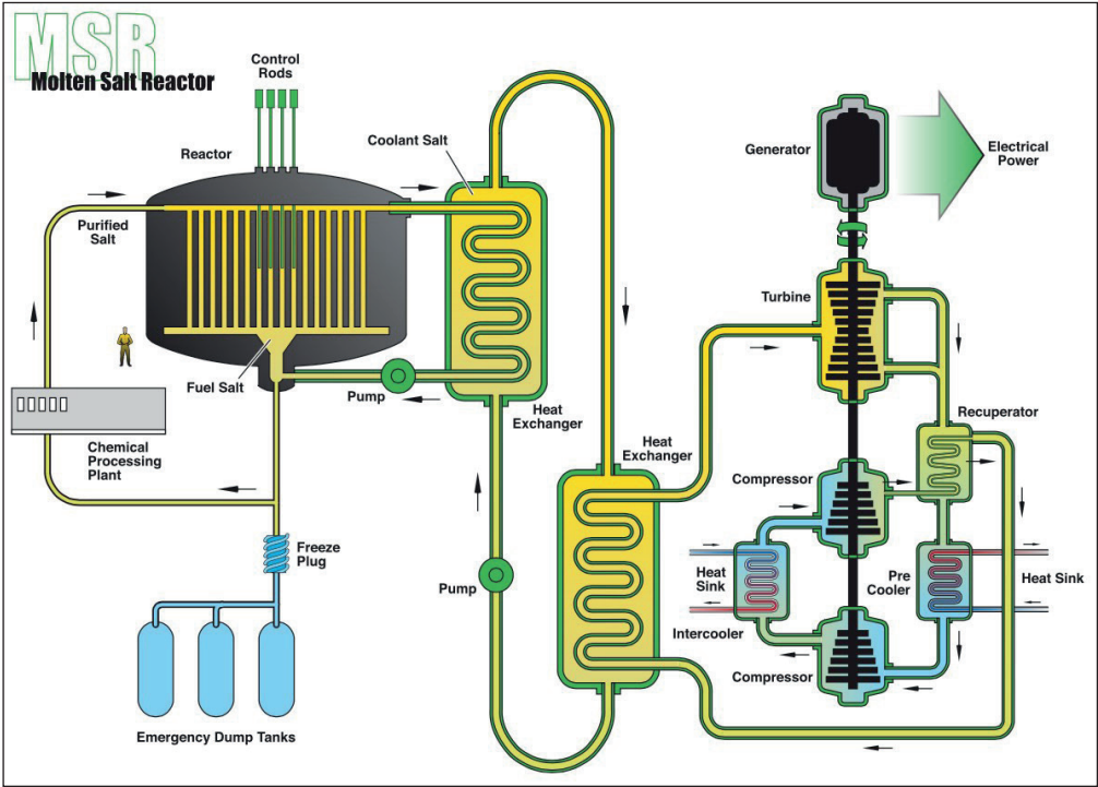
Figure 28: Molten Salt Reactor
