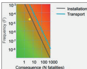
Figure 31: FN-curve
