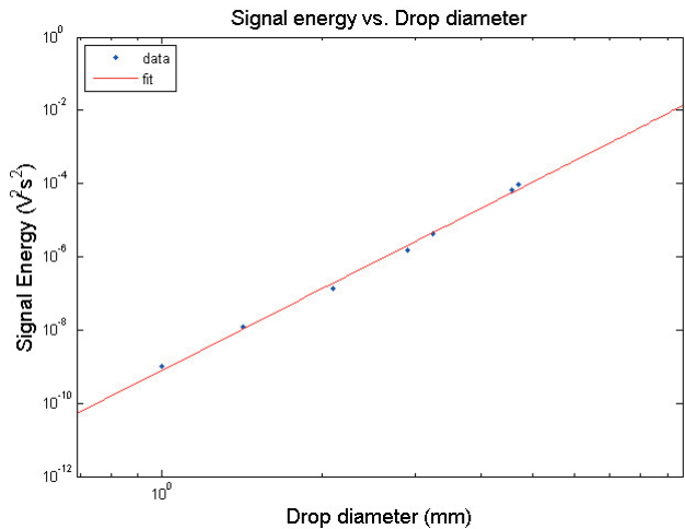
Figure 16: correlation between drop size and signal strength
