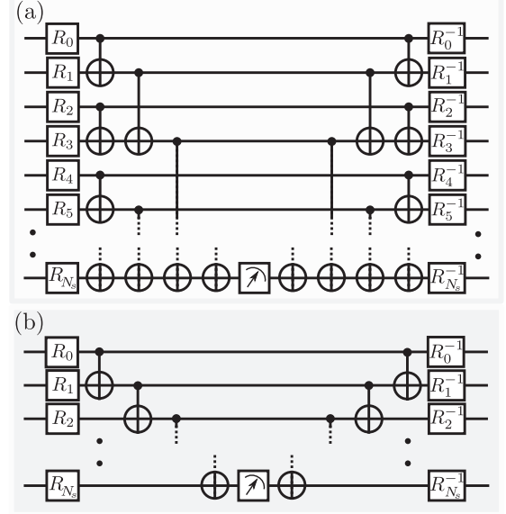
FIG. 2. Quantum circuits for in-line symmetry verification. (a) The optimal verification circuit has O(\log(N_S)) depth, but requires long-range connectivity between qubits, which is not available on many architectures. (b) In the presence of linear connectivity, an O(N_S) depth verification circuit is optimal.
