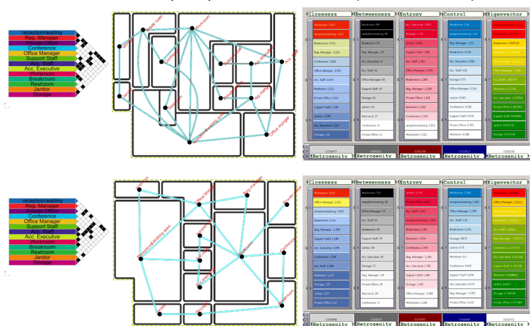
Figure 3.25 : The plans and centrality measures for both scenarios
