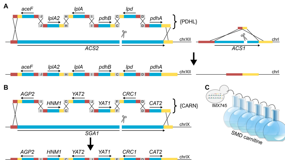
FIG 2 Construction of a lipophilic acid-dependent, carnitine shuttle-constitutive S. cerevisiae strain and its laboratory evolution for lipophilic acid-independent, carnitine-dependent growth. (A) In a previous study (33), the {PDHL} cluster, consisting of six cassettes required for cytosolic expression of a functional Enterococcus faecalis pyruvate dehydrogenase complex and flanked by 60-bp sequences, was assembled in vivo via homologous recombination (indicated with black crosses) and introduced into ACS2 after introduction of a Cas9-induced double-strand break. ACS1 was removed using a 120-bp DNA repair fragment (figure adapted from reference 33). (B) In this strain, the {CARN} cluster, consisting of six cassettes for constitutive expression of carnitine shuttle genes, was similarly in vivo assembled and introduced into the SGA1 locus, resulting in strain IMX745 ( acs1Δ acs2Δ:: {PDHL} sga1Δ:: {CARN}). Activity of the E. faecalis PDH in the yeast cytosol is lipophilic acid dependent (31). (C) As strain IMX745 did not show L-carnitine-dependent growth when lipophilic acid was omitted from growth media, an evolution experiment was initiated using synthetic medium with 20 g · liter -1 glucose (dextrose) (SMD) and 400 mg · liter -1 L-carnitine. Abbreviations: chrI, chromosome I; chrIX, chromosome IX; chrXII, chromosome XII.
