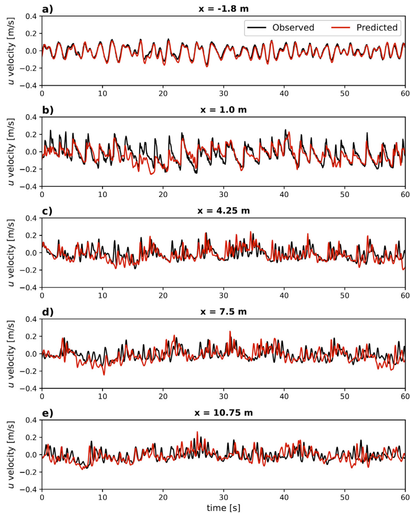
Fig. 10. Comparison of the velocity timeseries (illustrative 60 s period shown) between observations and predictions at 5 locations in the model domain where velocity measurements were available.
