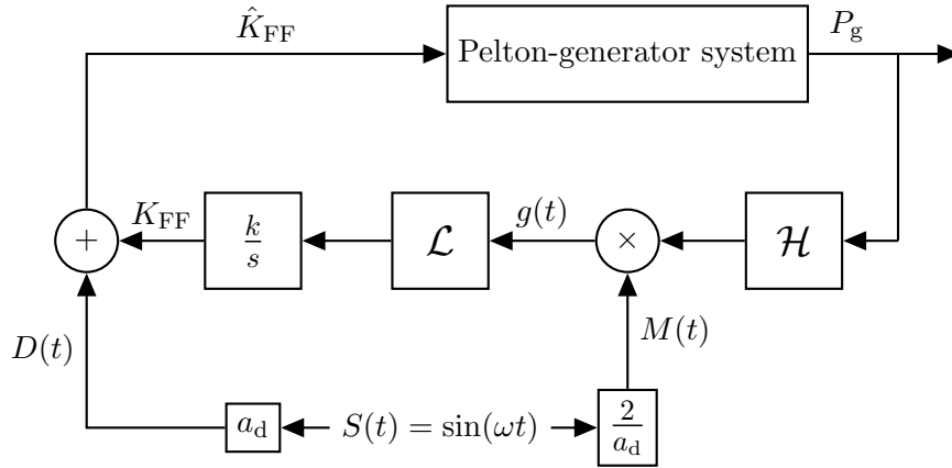
Figure 5: Block diagram of ESC implemented on the Pelton-generator system. The feed-forward gain K_{FF} is excited by the dither signal D(t) , and M(t) is used for demodulation of the high-pass filtered generator power output signal P_g . After demodulation, the gradient information of \partial P_g / \partial K_{FF} is contained as a DC-contribution in g(t) , which is subsequently low-pass filtered and integrated to arrive at the optimal value for K_{FF} .
