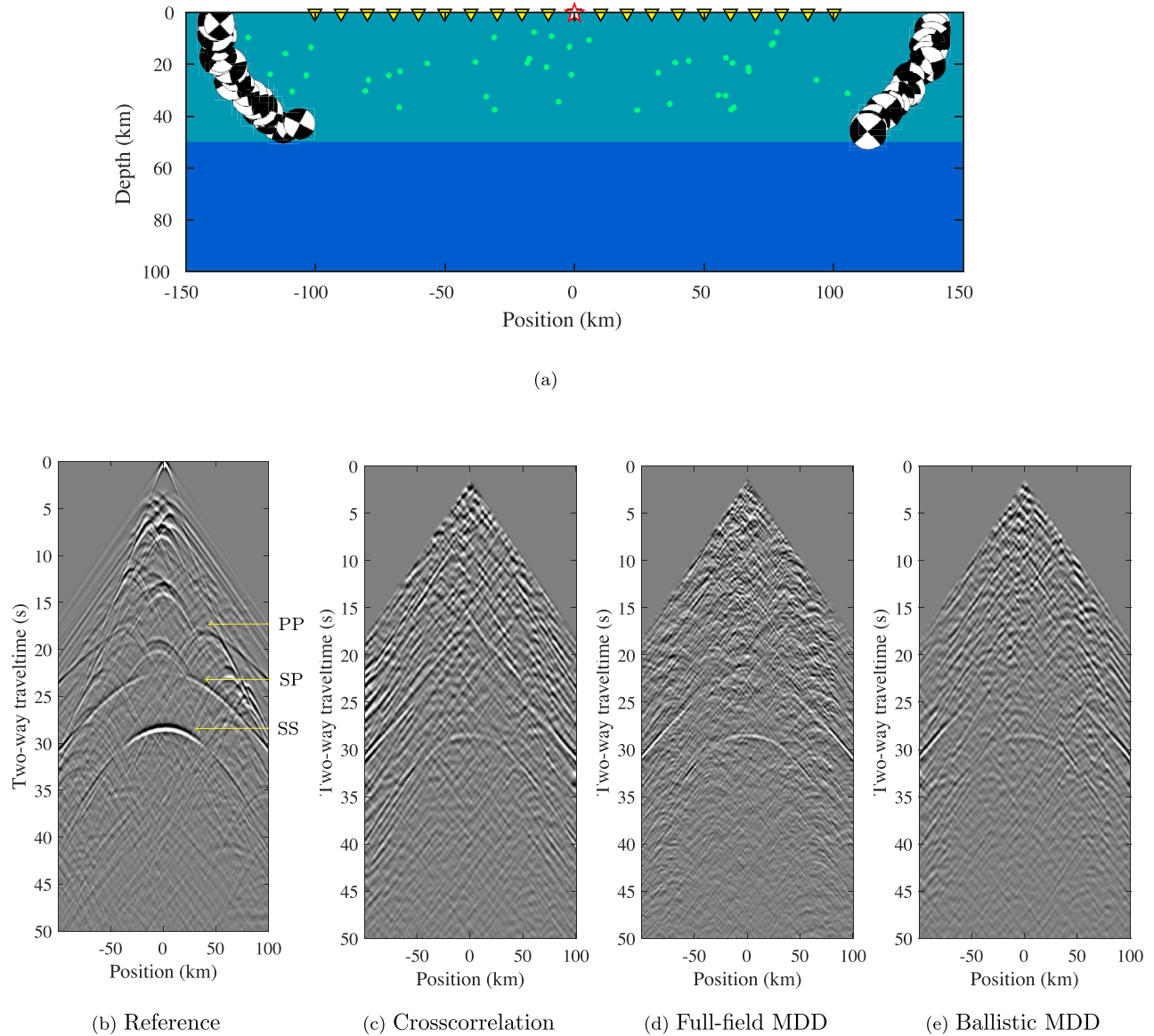
Figure 5. As Fig. 2, but with 50 scatterers in the crust.
