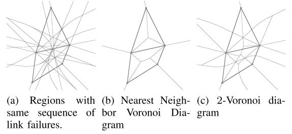
Fig. 7. An example of different partitions of the plane into regions used in Lemma 1.
