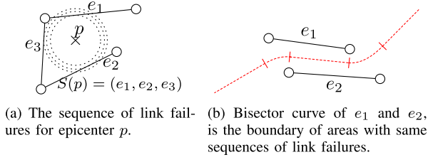
Fig. 6. Illustration of link failure sequences.
