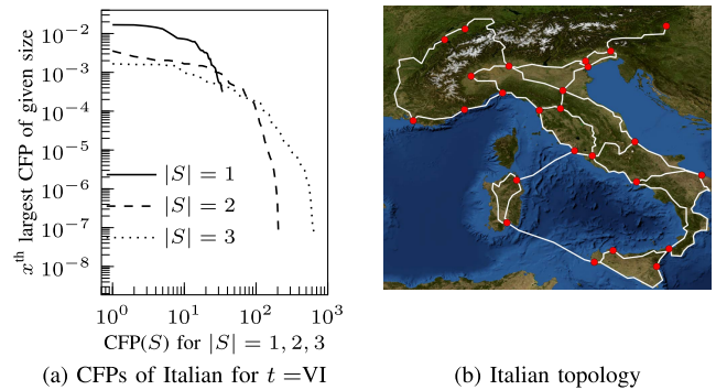
Fig. 11. CFP comparison of single, double and triple link failures for Italia.
