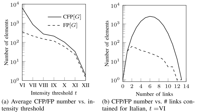
Fig. 10. Comparison of space efficiency of structures CFP[G] and FP[G].
