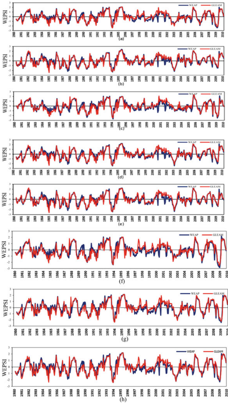
Fig. 10.4 Annual time series of GLEAM- and WEAP-based WEPSI06 in the sub-basins. a Acelhuate, b Guajillo, c Lempa1, d Lempa2, e Lempa3, f SS3, g SS6, and h Suquioyo
