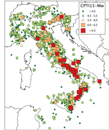
Fig. 2. Historical earthquakes from the most recent version of the historical parametric Italian catalogue [14]. M_w = moment magnitude.
