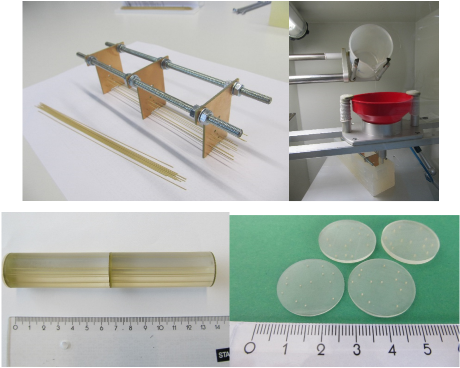
Figure 11: Fibre composite disc production: top left putting the sintered piezo fibres into the mask, top right: filling the mould with epoxy as substrate, bottom left: cured and mround milled rod, bottom right: sawed to four different thicknesses piezo discs
