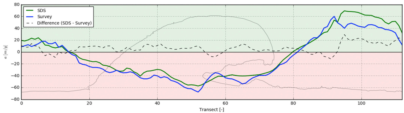
Fig. 14. Alongshore rate of shoreline change ( a ) based on the SDS position (green) and the survey MSL contour (blue). The black line indicates the difference between a_{SDS} and a_{Survey} . The MSL contour line from the survey conducted on 03-08-2011 is plotted in grey as a reference. (For interpretation of the references to colour in this figure legend, the reader is referred to the Web version of this article.)
