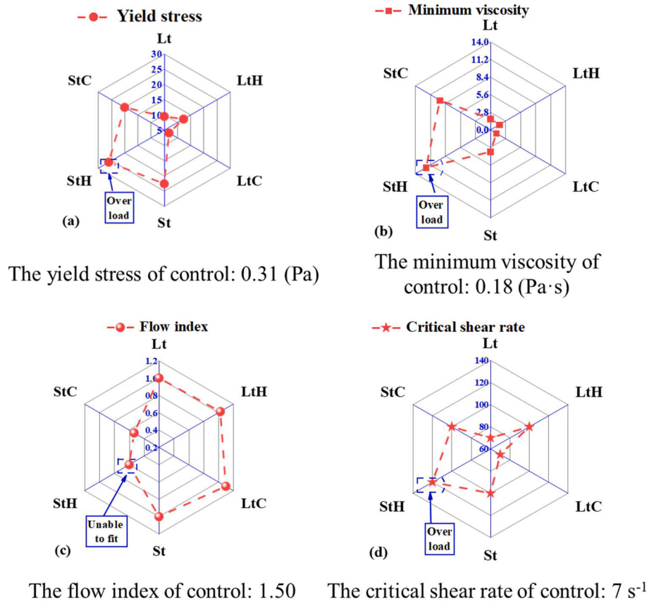
Fig. 6. Comparison of cement pastes containing various CNT with a diameter of 5 ~ 15 nm: (a) Yield stress \tau_0 ; (b) Minimum viscosity \eta_{\min} ; (c) Flow index n ; (d) Critical shear rate \gamma_{\text{cri}}
