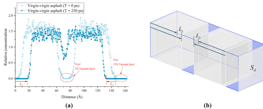
Fig. 10. The analysis and evaluation of asphalt diffusion model along the OZ direction: (a) relative concentration of virgin-virgin diffusion model; (b) principle of volume diffusion coefficient calculation.
