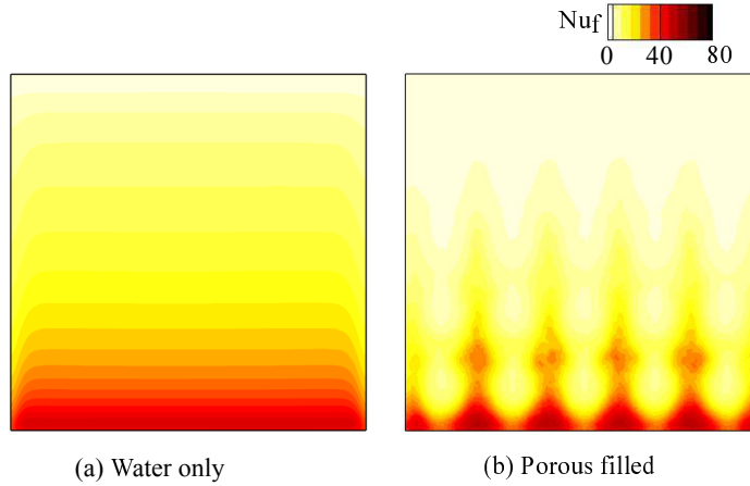
Figure 4.4: Nusselt number contour on the right wall in a water-only (a) and porous media filled (b) cavity, with constant temperature of \theta_l = 0 and \theta_r = 1 , at Ra_f = 10^7 . The contours are represented using a linear scale with 30 contour levels.
