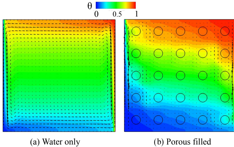
Figure 4.6: Non-dimensional temperature contours and velocity vectors in a vertical plane at X/L = 0.41 in a water-only (a) and porous media filled (b) cavity, with constant temperature \theta_l = 0 and \theta_r = 1 , at Ra_f = 10^7 . The contours are represented using a linear scale with 30 contour levels.
