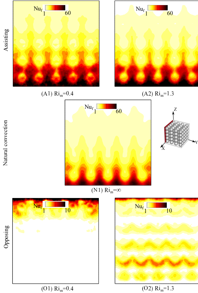
Figure 5.5: Instantaneous Nusselt number Nu_f distributions at the hot wall in a cavity packed with hydrogel beads, at Ra_f = 10^7 , at different Ri_m in assisting mixed convection (top row), natural convection (center) and opposing mixed convection (bottom row). The Nu_f distributions reported are at t/t_0 = 30 , after a quasi steady-state has been reached.
