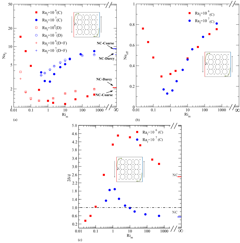
Figure 5.4: Heat transfer and thermal boundary layer thickness variation in a coarse-grained porous media filled cavity with opposing mixed convection, at different Ra_f and Ri_m . Solid dash indicate the heat transfer in the hydrogel bead filled cavity with natural convection at Ra_f = 10^6 (red), Ra_f = 10^7 (blue) (a) total heat transfer (b) scaled effective heat transfer (c) boundary layer thickness in coarse-grained filled cavity.
