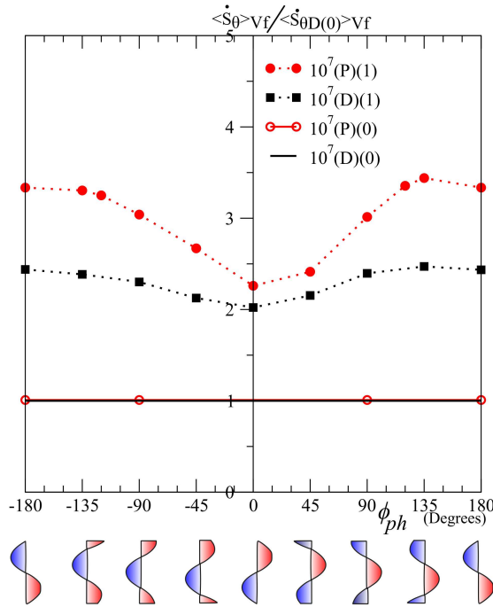
Figure 4.14: Variation of non-dimensional entropy generation of fluid due to temperature gradient with phase angle at Ra_f = 10^7 , with SWT ( \theta_l^{amp} = 1 ) and CWT ( \theta_l^{amp} = 0 ) in a water-only (D) and porous media filled (P) cavity.
