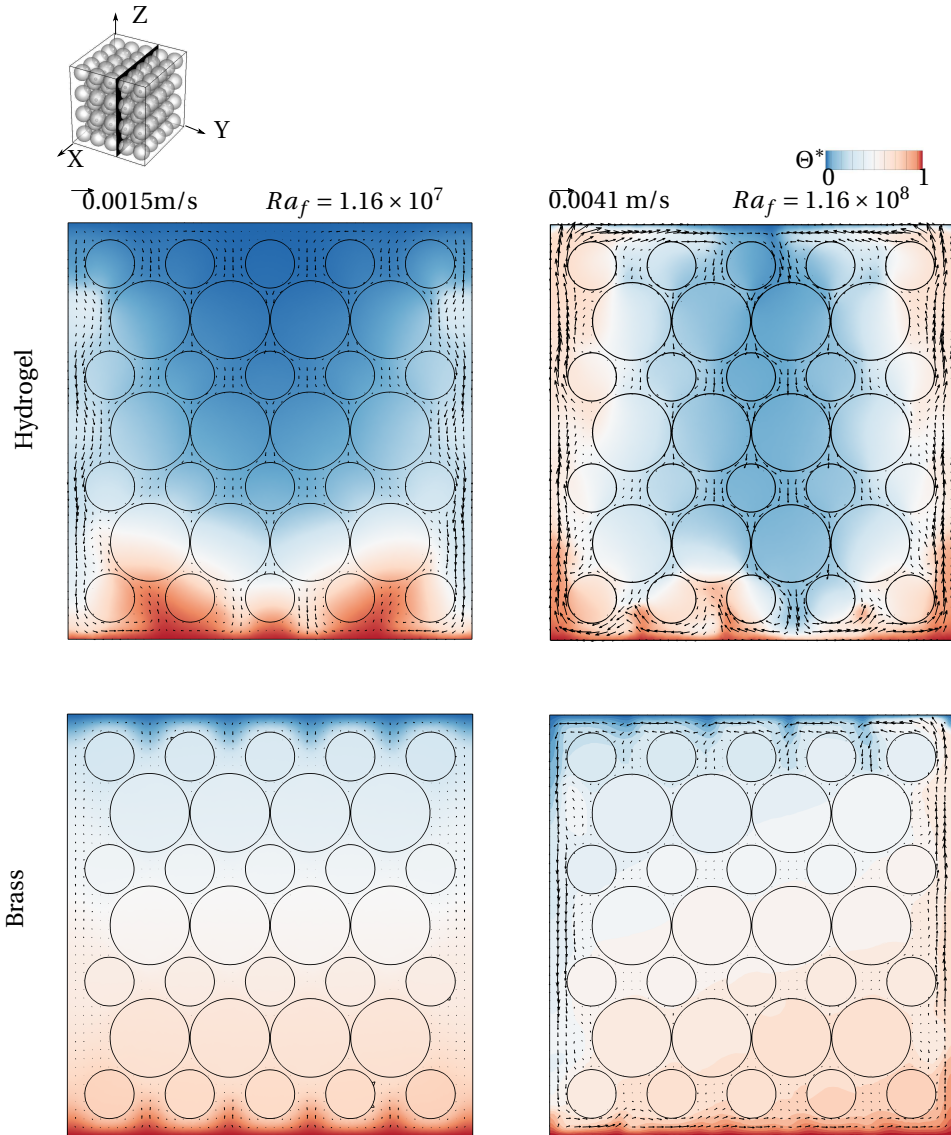
Figure 3.2: Instantaneous velocity vectors and temperatures at t/t_0 = 20 , in a characteristic vertical plane at Y/L = 0.62 at Ra_f = 1.16 \times 10^7 (left) and Ra_f = 1.16 \times 10^8 (right), for a cavity packed with hydrogel (top) and brass (bottom) beads.
