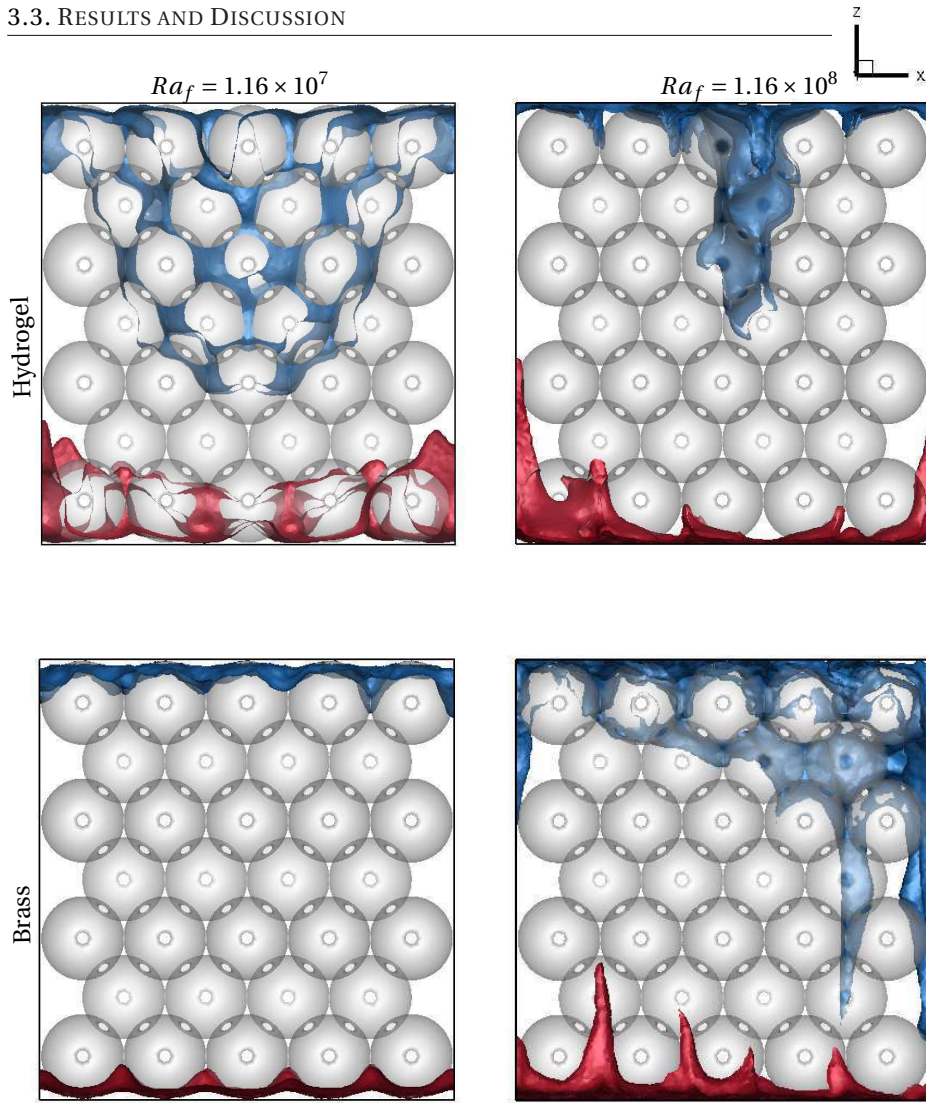
Figure 3.1: A side-view of the instantaneous non-dimensional temperature isosurfaces at t/t_0 = 20 , in a cavity filled with hydrogel (top) and brass (bottom) beads at Ra_f = 1.16 \times 10^7 (left) and Ra_f = 1.16 \times 10^8 (right) ( \Theta^* = 0.2 , Blue; \Theta^* = 0.8 , Red)
