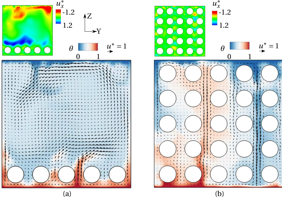
Figure 2.10: Instantaneous non-dimensional temperature distribution and velocity vectors at x/L = 0.43 , in a cavity with (a) 1 layer, (b) 5 layers of spherical beads at Ra = 2.3 \times 10^7 . The smaller figure to the left of temperature contour depicts the non-dimensional out of plane velocity. The velocity vectors are visualized by projecting them to a 32 \times 32 grid along the vertical plane.
