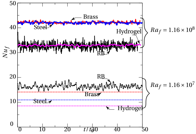
Figure 3.7: Time evolution of instantaneous, bottom wall-averaged, Nusselt number for cavities packed with brass (red), steel (blue) and hydrogel (magenta) beads, as well as for RB convection (black) at Ra_f = 1.16 \times 10^7 (dashed) and 1.16 \times 10^8 (solid).
