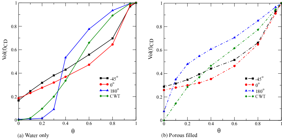
Figure 4.11: Cumulative distribution (discrete) of the fraction of fluid volume where \theta \leq \zeta\theta_{max} , in water-only (a) and porous media filled (b) cavities, with the left wall having a sinusoidal temperature distribution with amplitude \theta_l^{amp} = 1 at \phi_{ph} = -45^\circ (black), \phi_{ph} = 0^\circ (red), \phi_{ph} = 180^\circ (blue) at Ra_f = 10^7 . The results are compared with the respective cavities at constant wall temperature (green).
