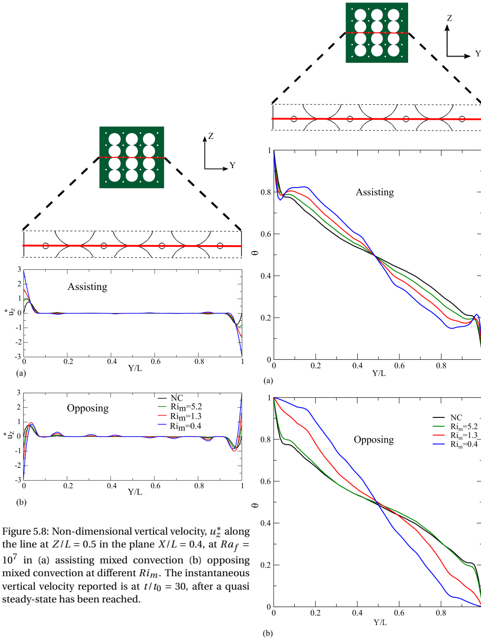
Figure 5.9: Non-dimensional temperature along the line at Z/L = 0.5 in the plane X/L = 0.4 , at Ra_f = 10^7 in (a) assisting mixed convection (b) opposing mixed convection at different Ri_m . The instantaneous temperature reported is at t/t_0 = 30 , after a quasi steady-state has been reached.
