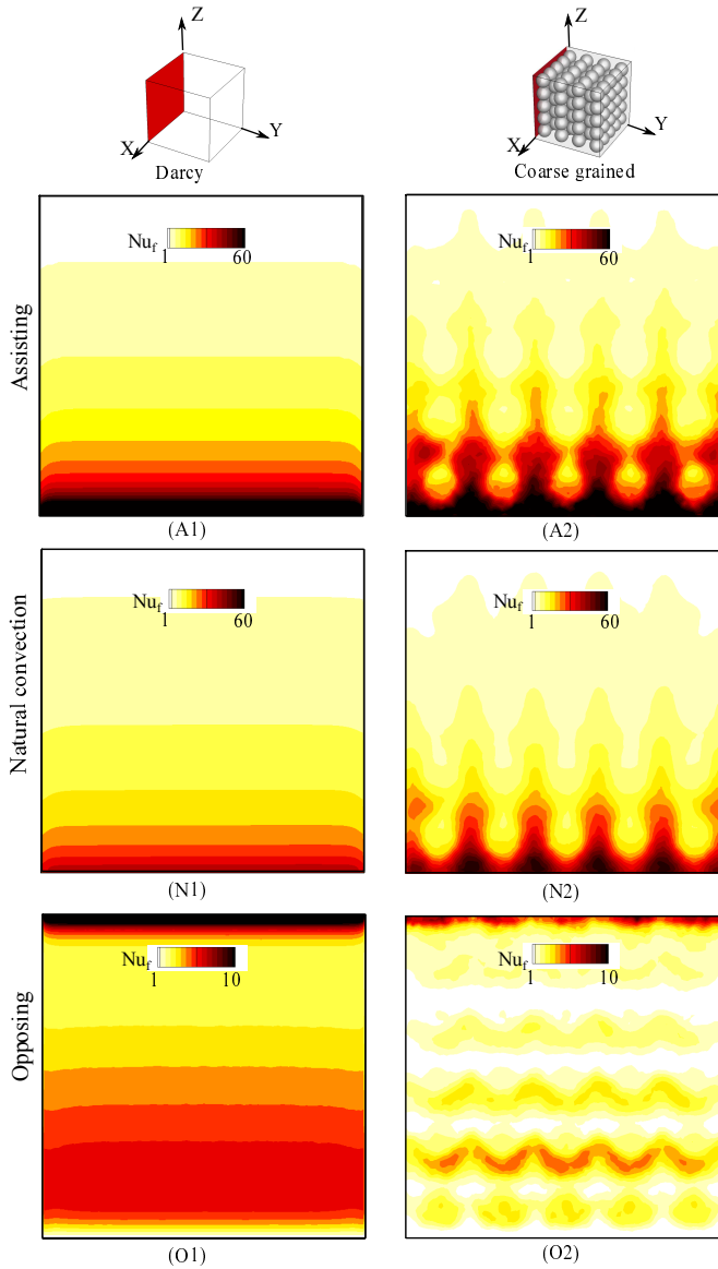
Figure 5.6: Instantaneous Nusselt number Nu_f distributions at the hot wall at Ra_f = 10^7 , Ri_m = 1.3 in assisting mixed convection (top row), natural convection (center) and opposing mixed convection (bottom row), with Darcy ( D ) assumption (left column) and coarse-grained ( C ) porous media filled cavity (right column). The Nu_f distributions reported are at t/t_0 = 30 , after a quasi steady-state has been reached.
