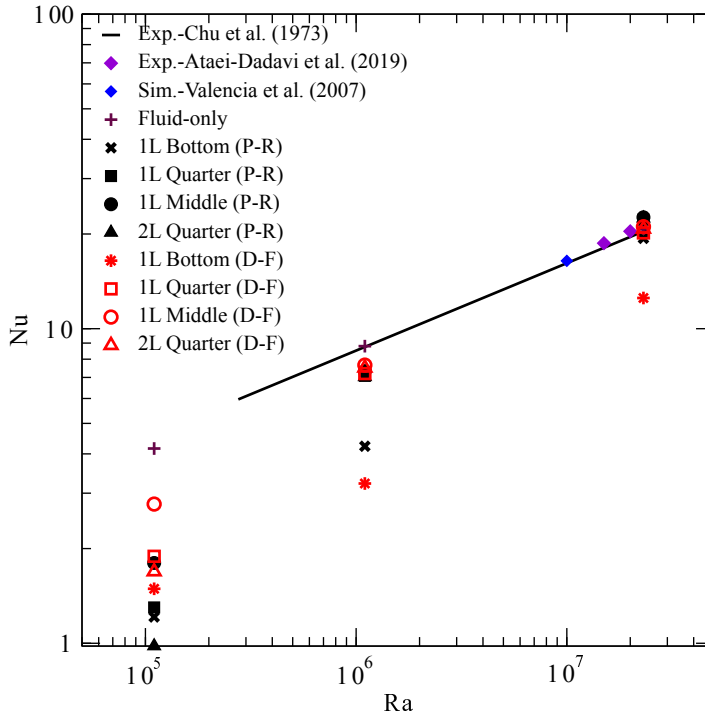
Figure 2.12: Variation of Nu with Ra in pore-structure resolved (P-R) and Darcy-Forchheimer (D-F) simulations for different packing arrangement. The results are compared with heat transfer in fluid-only cavities reported in literature [21, 45, 46]. For naming convection of packing arrangement refer to Table 2.1.
