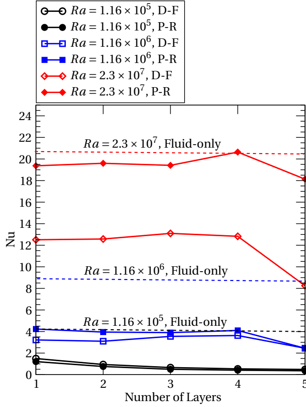
Figure 2.5: Variation of time- and wall- averaged Nusselt number with number of layers of packing at different Rayleigh numbers. A comparison of pore-structure resolved (P-R) simulations is made with that from Darcy-Forchheimer (D-F) simulations and fluid-only filled cavity.
