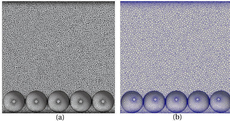
Figure 2.2: Cubical cavity packed with 1 layer of adiabatic spherical beads meshed using (a) tetrahedral grids (b) polyhedral grids.
