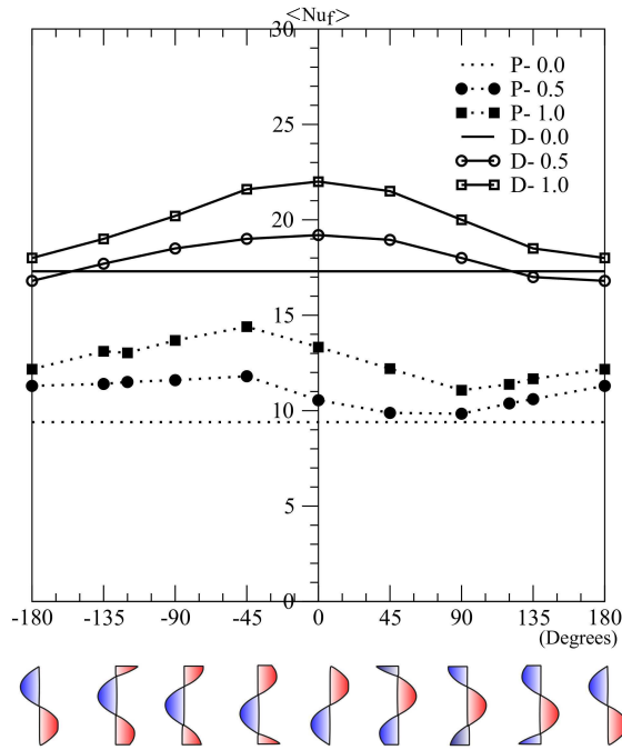
Figure 4.3: Variation of Nusselt number with phase angle at Ra_f = 10^7 and different amplitudes, \theta_l^{amp} (0, 0.5, 1) of cold wall temperature variation in a differentially heated water-only cavity (D) and porous media filled-cavity (P).
