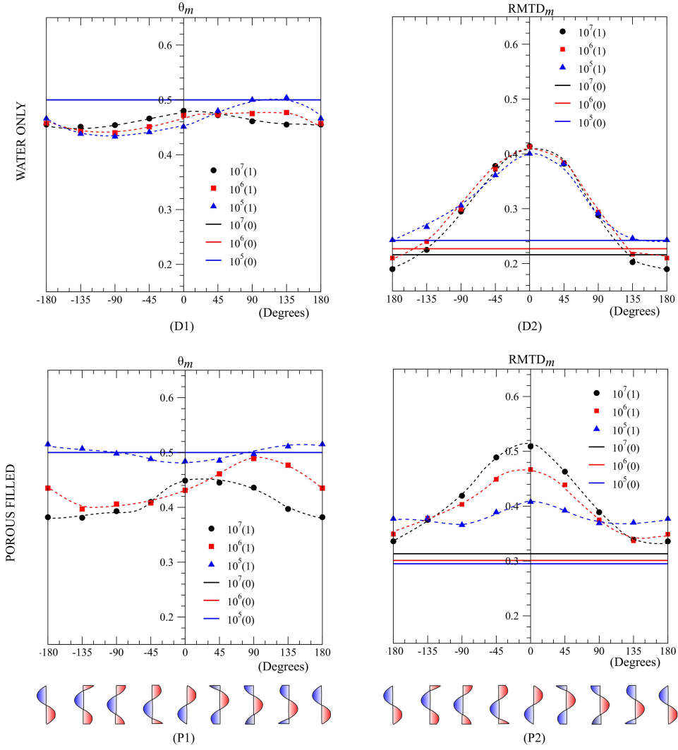
Figure 4.10: Variation of non-dimensional volume-averaged mean temperature ( D1 , P1 ) and RTD_m ( D2 , P2 ) of the fluid, with phase angle at different Rayleigh numbers ( Ra_f = 10^5, 10^6, 10^7 ) and different amplitudes (0, 1) of sinusoidal wall temperature in a water-only ( top row ) and porous media filled ( bottom row ) cavity. The dotted lines are only to guide the eyes.
