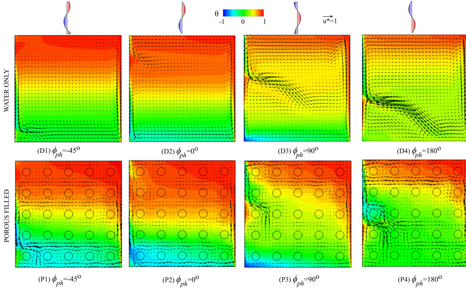
Figure 4.7: Non-dimensional temperature contours and velocity vectors in a vertical plane at X/L = 0.41 in a water-only ( top row ) and porous media filled ( bottom row ) cavities, with the left wall having a sinusoidal temperature distribution with amplitude \theta_l^{amp} = 1 and varying phase angle \Phi_{ph} , at Ra_f = 10^7 . The contours are represented using a linear scale with 30 contour levels.
