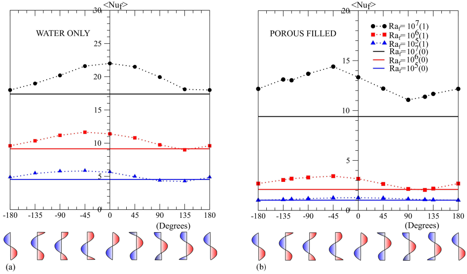
Figure 4.2: Variation of Nusselt number with phase angle at different Rayleigh numbers ( Ra_f = 10^5, 10^6, 10^7 ) and different amplitudes, \theta_l^{amp} = 0 (CWT), 1 in water-only (a) and porous media filled (b) cavity.
