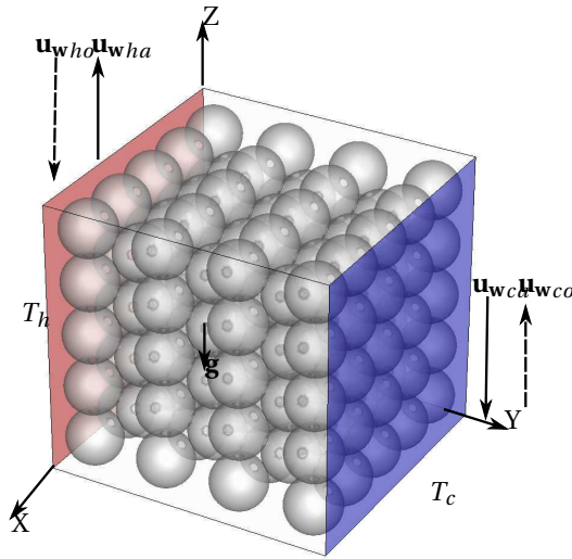
Figure 5.1: Schematic representation of a hydrogel bead filled side heated cavity with the side walls at temperature T_c and T_h . The arrows show the direction of moving wall.
