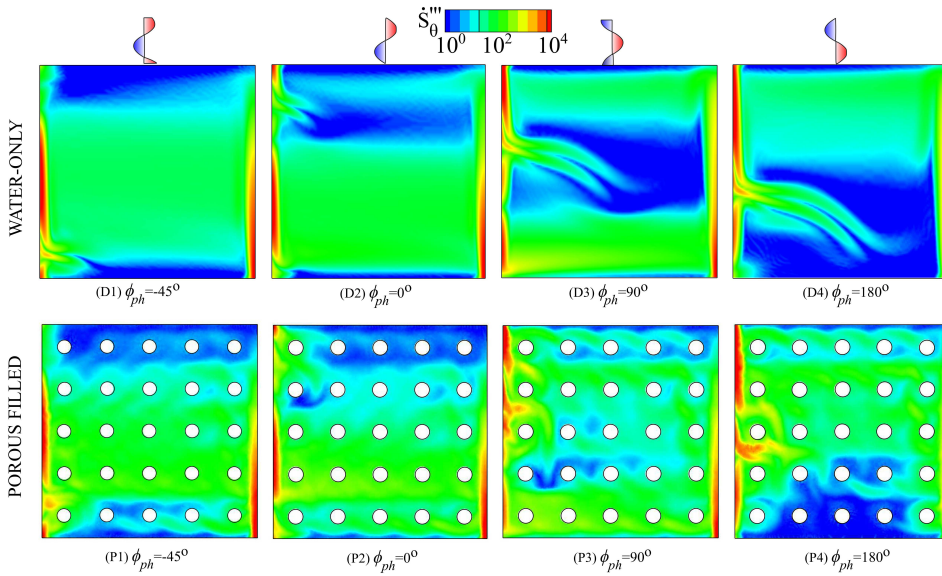
Figure 4.13: Entropy generated in the fluid region due to temperature gradient in a characteristic vertical plane at X/L = 0.41 in a water-only ( top row ) and porous media filled ( bottom row ) cavity, with the left wall having sinusoidal temperature distribution with amplitude \theta_l^{amp} = 1 and varying phase angle \Phi_{ph} , at Ra_f = 10^7 .
