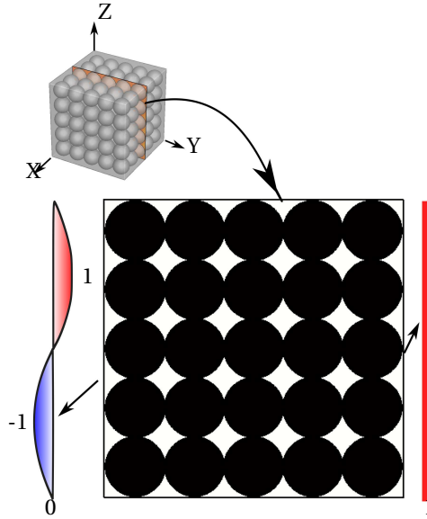
Figure 4.1: Geometrical representation of the differentially heated water filled cavity with hydrogel beads. The left wall has a sinusoidal non-dimensional temperature, \theta_r = 1 , with \theta_l = 0 and \theta_l^{amp} = 1 .
