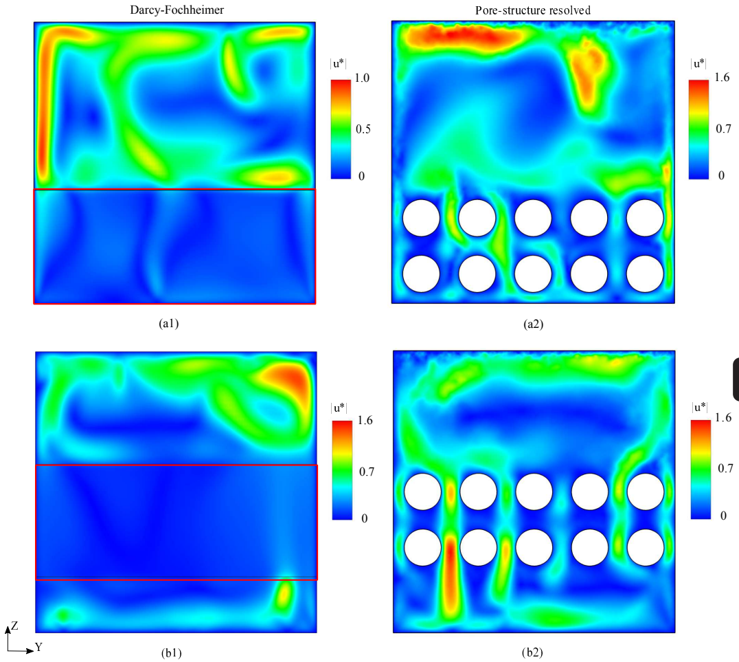
Figure 2.14: Instantaneous non-dimensional velocity magnitude distribution at x/L = 0.43 , in a cavity with 2 layers of spherical beads at Ra = 2.3 \times 10^7 in Darcy-Forchheimer (a1,b1) and pore-structure resolved (a2,b2) simulations. (a1,a2) has porous media from z/L = 0 to 0.4 and (b1, b2) has porous media from z/L = 0.2 to 0.6.
