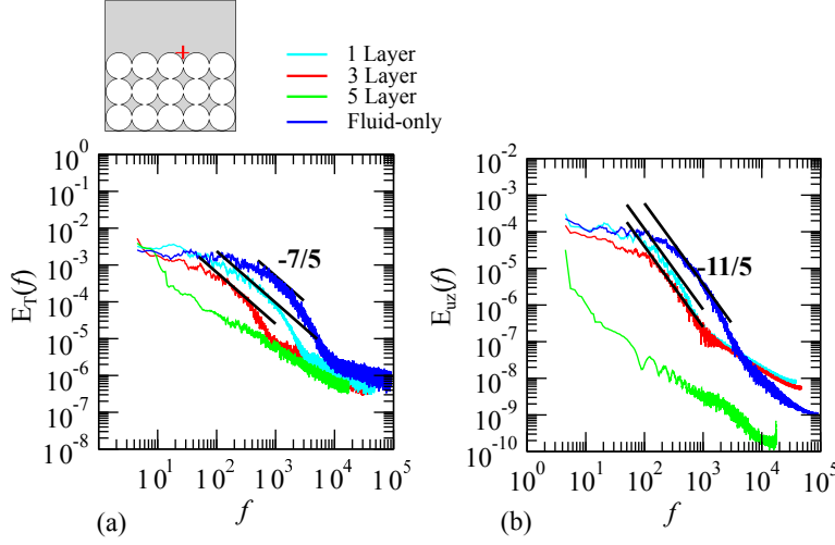
Figure 2.11: Power-laws for the frequency (a) thermal energy spectra and (b) kinetic energy spectra of the vertical velocity u_z at Ra = 2.3 \times 10^7 , y/L = 0.5 , x/L = 0.6 , z/L = 0.6 .
