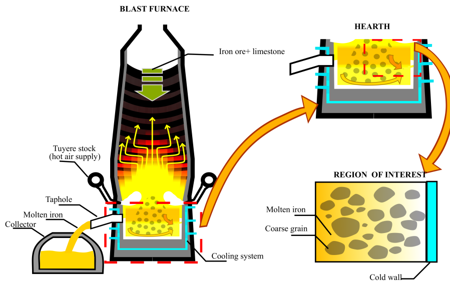
Figure 1.1: Schematic representation of a blast furnace. The image is an adapted version available in [1]. The hearth of the blast furnace is simplified as a side-heated side-cooled cavity filled with porous media.
