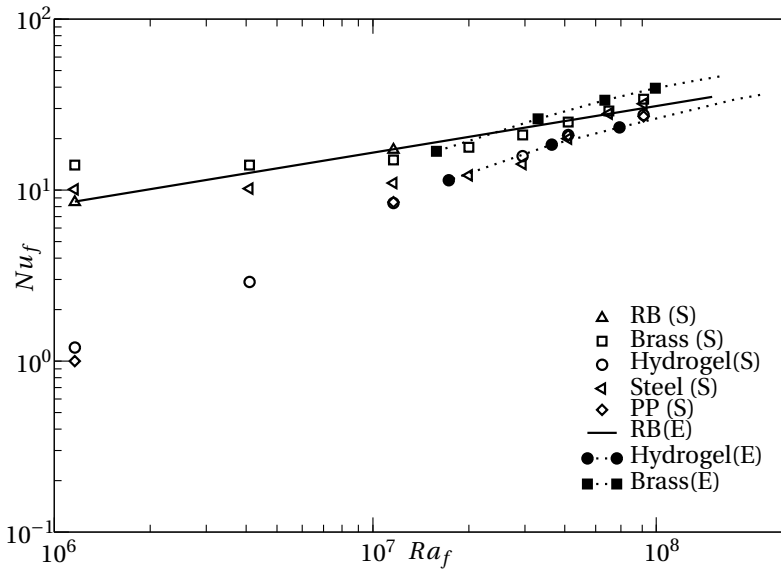
Figure 3.8: Simulated and experimental ([14]) long-term time-and-wall-averaged Nusselt numbers as a function of Rayleigh number for 1.16 \times 10^6 \leq Ra_f \leq 1.16 \times 10^8 in cavities packed with polypropylene (PP), hydrogel, steel and brass, as well as in RB convection. The solid line represents the Nu_f - Ra_f relation obtained experimentally for RB convection and the dotted lines connecting the symbols represent the asymptotic behavior of Nu_f with increase in Ra_f for different packing materials.
