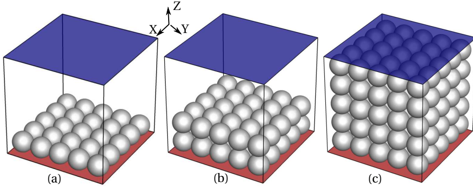
Figure 2.1: Geometrical representation of fluid-filled cubical cavity heated from the bottom (red) and cooled from the top (blue) packed with (a) 1 layer (b) 2 layers (c) 5 layers of adiabatic spherical beads.
