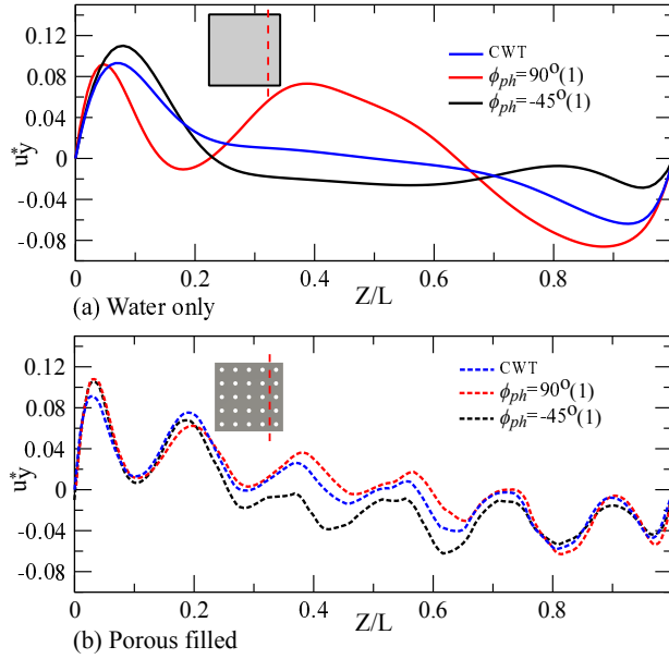
Figure 4.9: Non-dimensional horizontal velocity ( u_y^* ) along the vertical line Y/L = 0.8 , in a vertical plane at X/L = 0.41 in water-only (a) and porous media filled (b) cavities, with the left wall having a sinusoidal temperature distribution with amplitude \theta_l^{amp} = 1 at \phi_{ph} = 90^\circ (red) and -45^\circ (black), at Ra_f = 10^7 . The results are compared with the respective cavities at constant wall temperature (blue).
