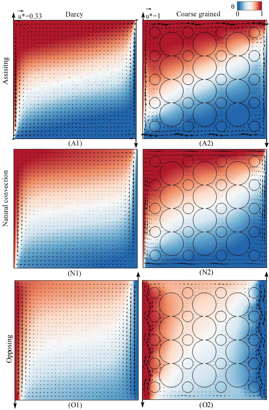
Figure 5.7: Instantaneous velocity vectors and temperatures in a characteristic vertical plane, X/L = 0.79 at Ra_f = 10^7 , Rl_m = 1.3 in assisting mixed convection (top row), natural convection (center) and opposing mixed convection (bottom row) with Darcy (D) assumption (left column) and coarse-grained (C) porous media filled cavity (right column). The instantaneous data reported is at t/t_0 = 30 , after a quasi steady-state has been reached.
