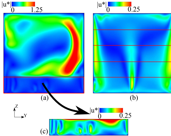
Figure 2.8: Instantaneous non-dimensional velocity magnitude distribution at x/L = 0.43 , in a cavity with (a) 1 layer (b) 5 layers at Ra = 2.3 \times 10^7 simulated using Darcy-Forchheimer assumption. The legend of (c) has a different scale from (a).
