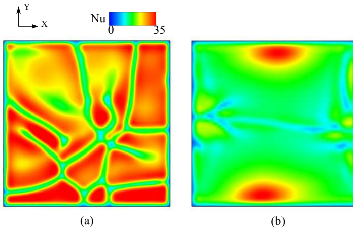
Figure 2.6: Instantaneous Nusselt number distribution (top view) at the bottom wall, in a cavity with porous media filled to a height equivalent to (a) 1 layer (b) 5 layers of spherical beads at Ra = 2.3 \times 10^7 obtained with Darcy-Forchheimer (D-F) simulations.
