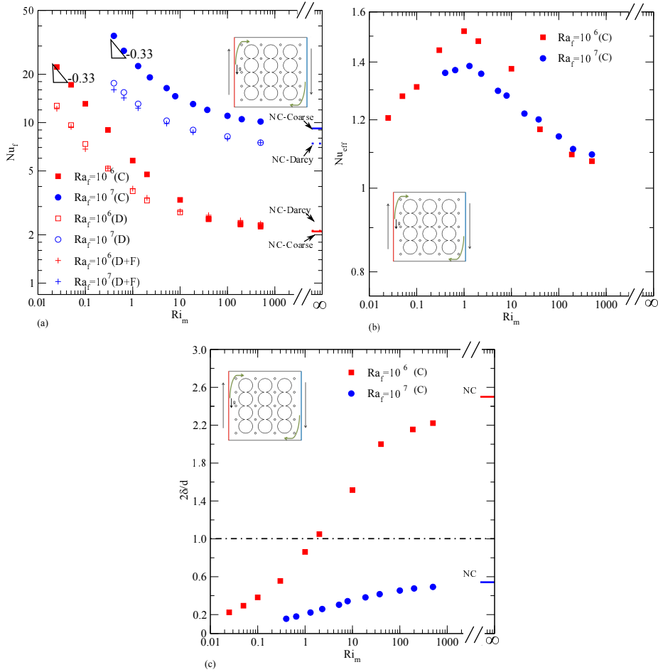
Figure 5.3: Heat transfer and thermal boundary layer thickness variation in a coarse-grained porous media filled cavity with assisting mixed convection, at different Ra_f and Ri_m . Solid dash indicate the heat transfer in the hydrogel bead filled cavity with natural convection at Ra_f = 10^6 (red), Ra_f = 10^7 (blue) (a) total heat transfer (b) scaled effective heat transfer (c) boundary layer thickness in coarse-grained filled cavity.
