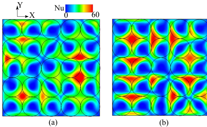
Figure 2.9: Instantaneous Nusselt number distribution (top view) at the bottom wall, in a cavity with (a) 1 layer (b) 5 layers of spherical beads at 2.3 \times 10^7 obtained with pore-structure resolved (P-R) simulations.
