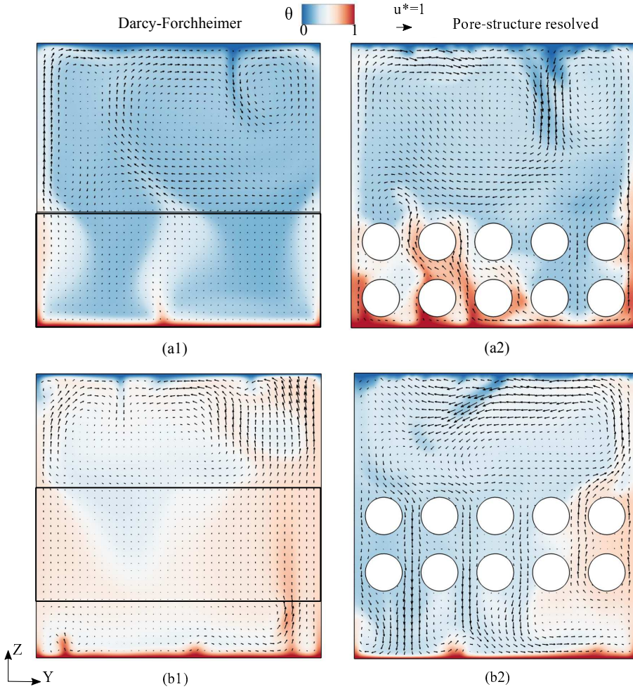
Figure 2.15: Instantaneous non-dimensional temperature distribution and velocity vectors at x/L = 0.43 , in a cavity with 2 layers of spherical beads at Ra = 2.3 \times 10^7 in Darcy-Forchheimer (a1,b1) and pore-scale resolved (a2,b2) simulations. (a1,a2) has porous media from z/L = 0 to 0.4 and (b1, b2) has porous media from z/L = 0.2 to 0.6 .
