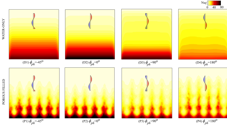
Figure 4.5: Nusselt number contour at the right wall in a water-only ( top row ) and porous media filled ( bottom row ) cavity, with the left wall having sinusoidal temperature distribution of amplitude \theta_l^{amp} = 1 and varying phase angle \Phi_{ph} , at Ra_f = 10^7 . The contours are represented using a linear scale with 30 contour levels.
