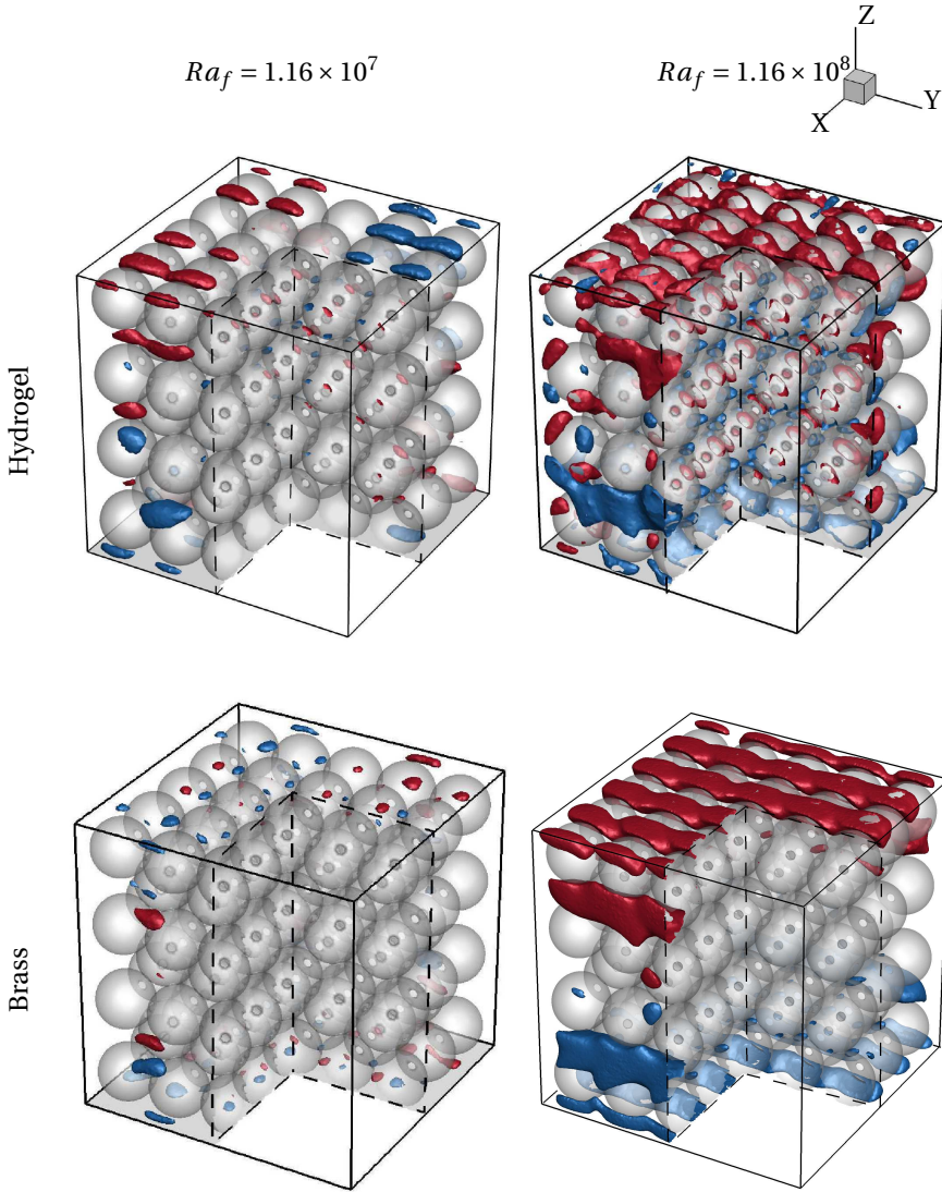
Figure 3.5: Instantaneous normalized lateral velocity isosurfaces, v^* = 0.2 (red) and v^* = -0.2 (blue) at t/t_0 = 20 , in a cavity packed with hydrogel (top) and brass (bottom) beads at Ra_f = 1.16 \times 10^7 (left) and 1.16 \times 10^8 (right).
