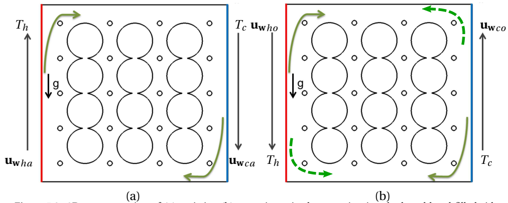
Figure 5.2: 2D representation of (a) assisting (b) opposing mixed convection in a hydrogel bead filled side heated cavity with the side walls at temperature T_c and T_h . In (a) solid arrows show the net flow due to forced and natural convection; in (b) dashed arrows and solid arrows show the direction of flow induced by forced convection and natural convection respectively.
