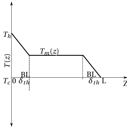
Figure A.1: Calculation of thermal boundary layer thickness from mean temperature profile for RBC convection. T(z) denotes the X-Y plane averaged temperature \langle T \rangle_{xy} at different height along the direction of gravity.
