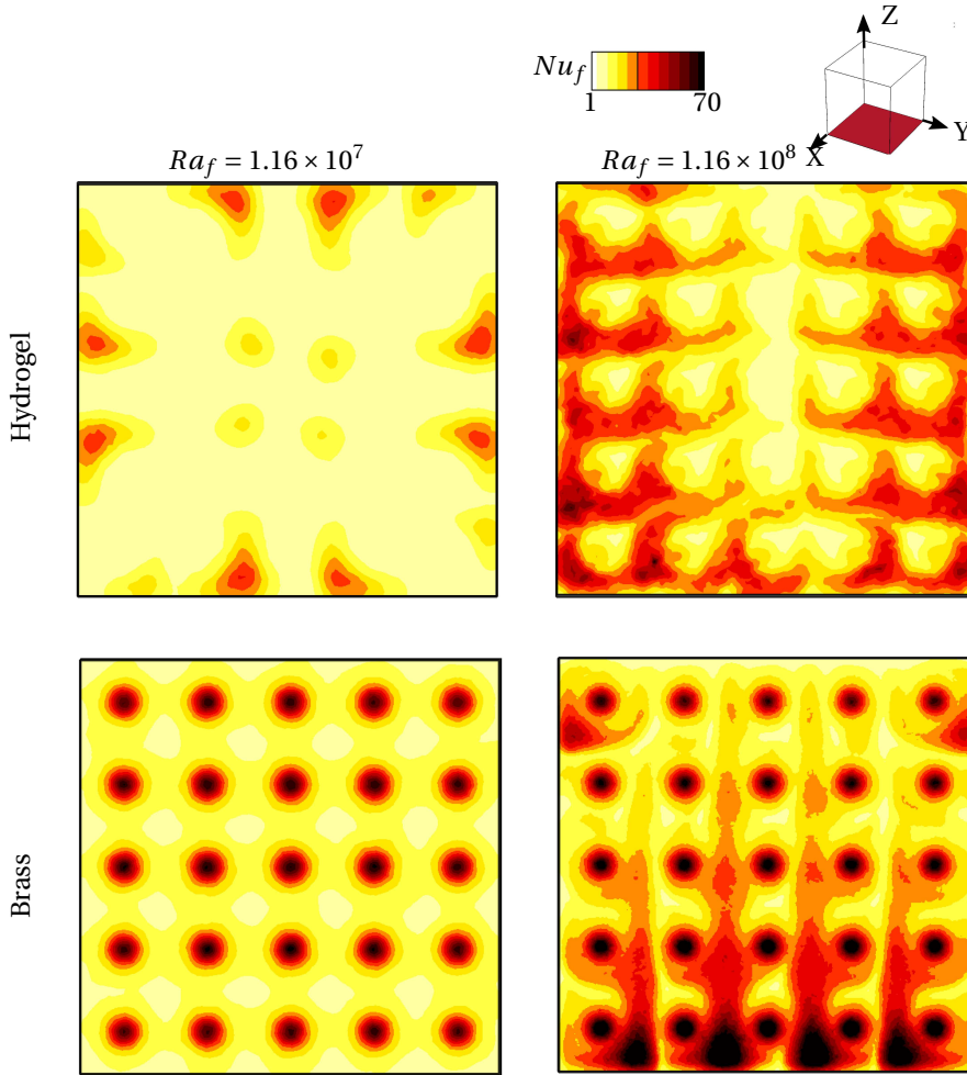
Figure 3.3: Instantaneous Nusselt number Nu_f distributions at the hot wall at t/t_0 = 20 , in a cavity packed with hydrogel (top) and brass (bottom) beads, at Ra_f = 1.16 \times 10^7 (left) and 1.16 \times 10^8 (right).
