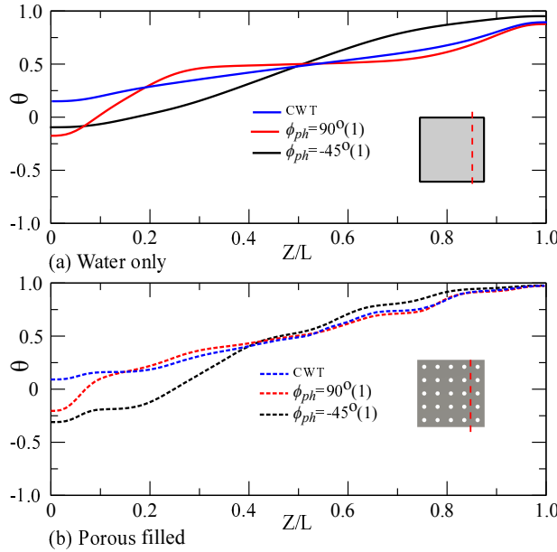
Figure 4.8: Non-dimensional temperature along the vertical line Y/L = 0.8 , in a vertical plane at X/L = 0.41 in water-only (a) and porous media filled (b) cavities, with the left wall having a sinusoidal temperature distribution with amplitude \theta_l^{amp} = 1 at \phi_{ph} = 90^\circ (red) and -45^\circ (black), at Ra_f = 10^7 . The results are compared with the respective cavities at constant wall temperature (blue).
