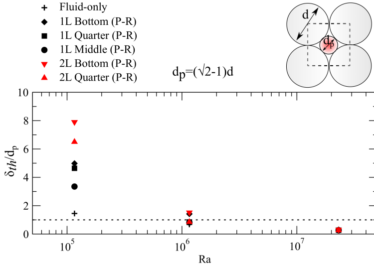
Figure 2.13: Ratio of boundary layer thickness to pore-size at different Ra , for pore-scale resolved simulations. The boundary layer thickness of fluid-only cavity is also scaled with pore-size of the porous media filled-cavity for reference.
