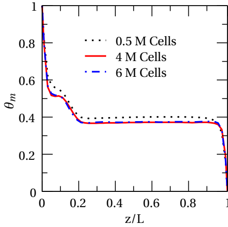
Figure 2.3: Time- and plane- averaged mean temperature variation along Z direction in a cavity filled with 1 layer of spherical adiabatic beads for different mesh sizes at Ra = 2.3 \times 10^7 .
