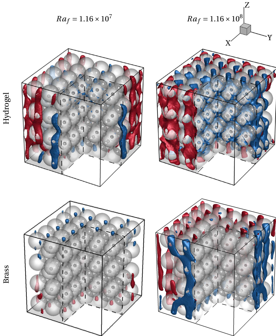
Figure 3.4: Instantaneous normalized vertical velocity isosurfaces, w^* = 0.2 (red) and w^* = -0.2 (blue) at t/t_0 = 20 , in a cavity packed with hydrogel (top) and brass (bottom) at Ra_f = 1.16 \times 10^7 (left) and 1.16 \times 10^8 (right).
