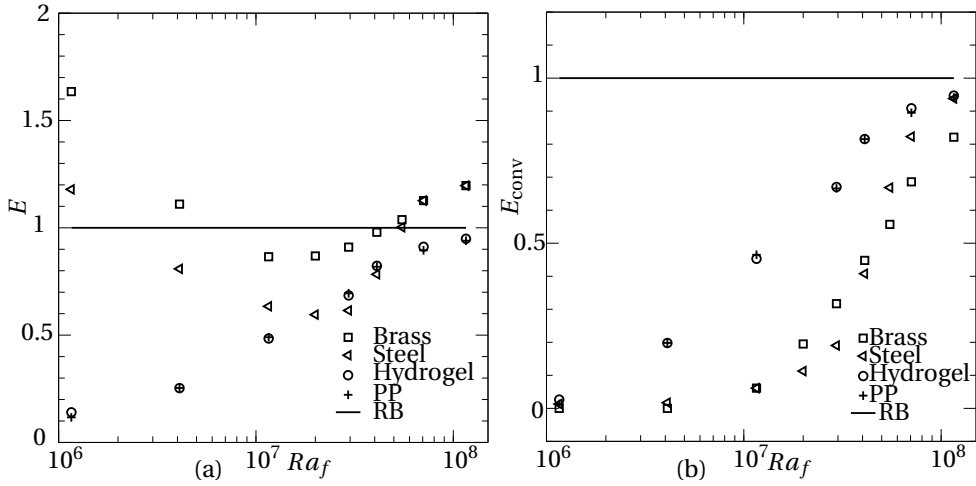
Figure 3.9: Heat transfer in a cavity packed with PP, hydrogel, steel and brass (a) scaled total heat transfer (b) scaled convective heat transfer.
