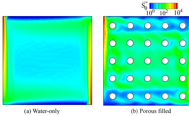
Figure 4.12: Entropy generated due to temperature gradient in the fluid region (log scale) in a characteristic vertical plane at X/L = 0.41 in a water-only (a) and porous media filled (b) cavity, with constant temperature left wall \theta_l = 0 and right wall temperature \theta_r = 1 , at Ra_f = 10^7 .
