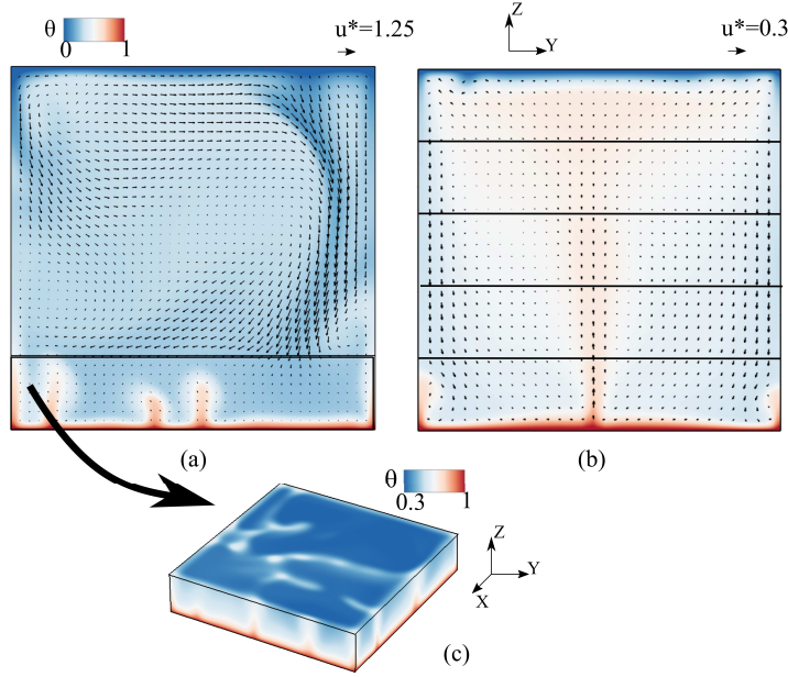
Figure 2.7: Instantaneous non-dimensional temperature distribution and velocity vectors at x/L = 0.43 , in a cavity with (a) 1 layer (layer height highlighted with a box) (b) 5 layers at Ra = 2.3 \times 10^7 simulated using Darcy-Forchheimer assumption. The velocity vectors are visualized by projecting them to a 32 \times 32 grid along the vertical plane. The enlarged 3D view of the temperature distribution in the porous region of cavity with 1 Layer of packing is depicted in (c) with a different colour scale.
