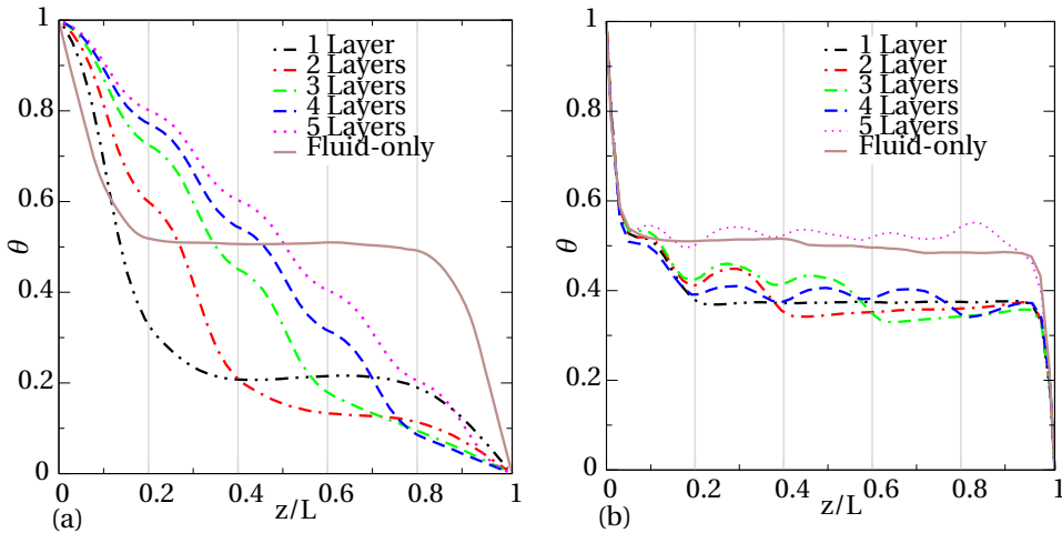
Figure 2.4: Time- and plane- averaged non-dimensional temperature for cavities filled with different layers of spherical bead packing at (a) Ra = 1.16 \times 10^5 , (b) Ra = 2.3 \times 10^7 . Plane-averaging along planes with adiabatic spheres results in the wavy temperature distribution. The deviation in mean temperature from \theta = 0.5 for 5 layer packing indicates the need of time averaging for longer period.
