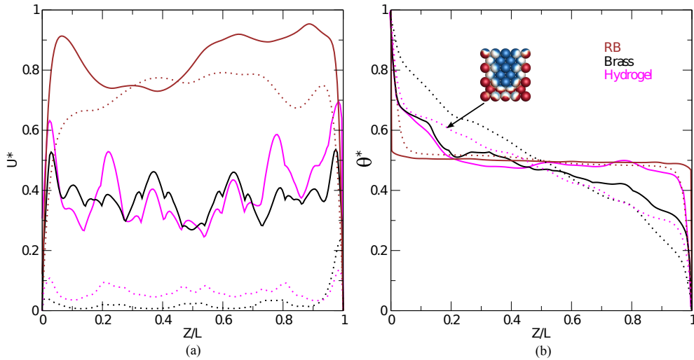
Figure 3.6: Instantaneous scaled velocity magnitudes U^* (a) and normalized temperatures \Theta^* (b) at t/t_0 = 20 , averaged over XY -planes as a function of Z/L , in RB convection (brown), hydrogel packed (pink) and brass packed (black) cavities at Ra_f = 1.16 \times 10^7 ( \cdots ) and 1.16 \times 10^8 (—). An example of the temperature distribution on the surface of the solid spheres is depicted in the inset.
