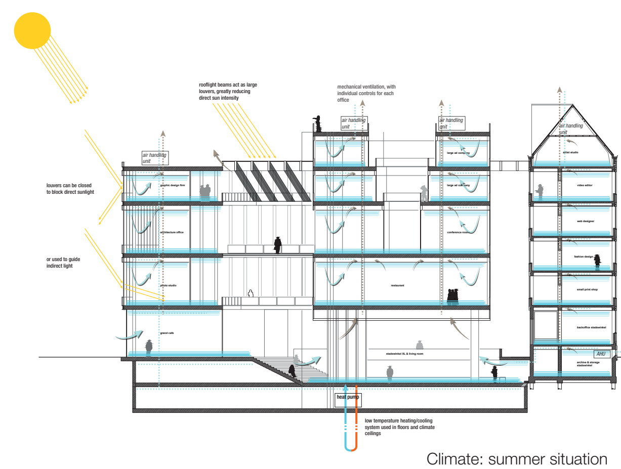
Climate: summer situation
