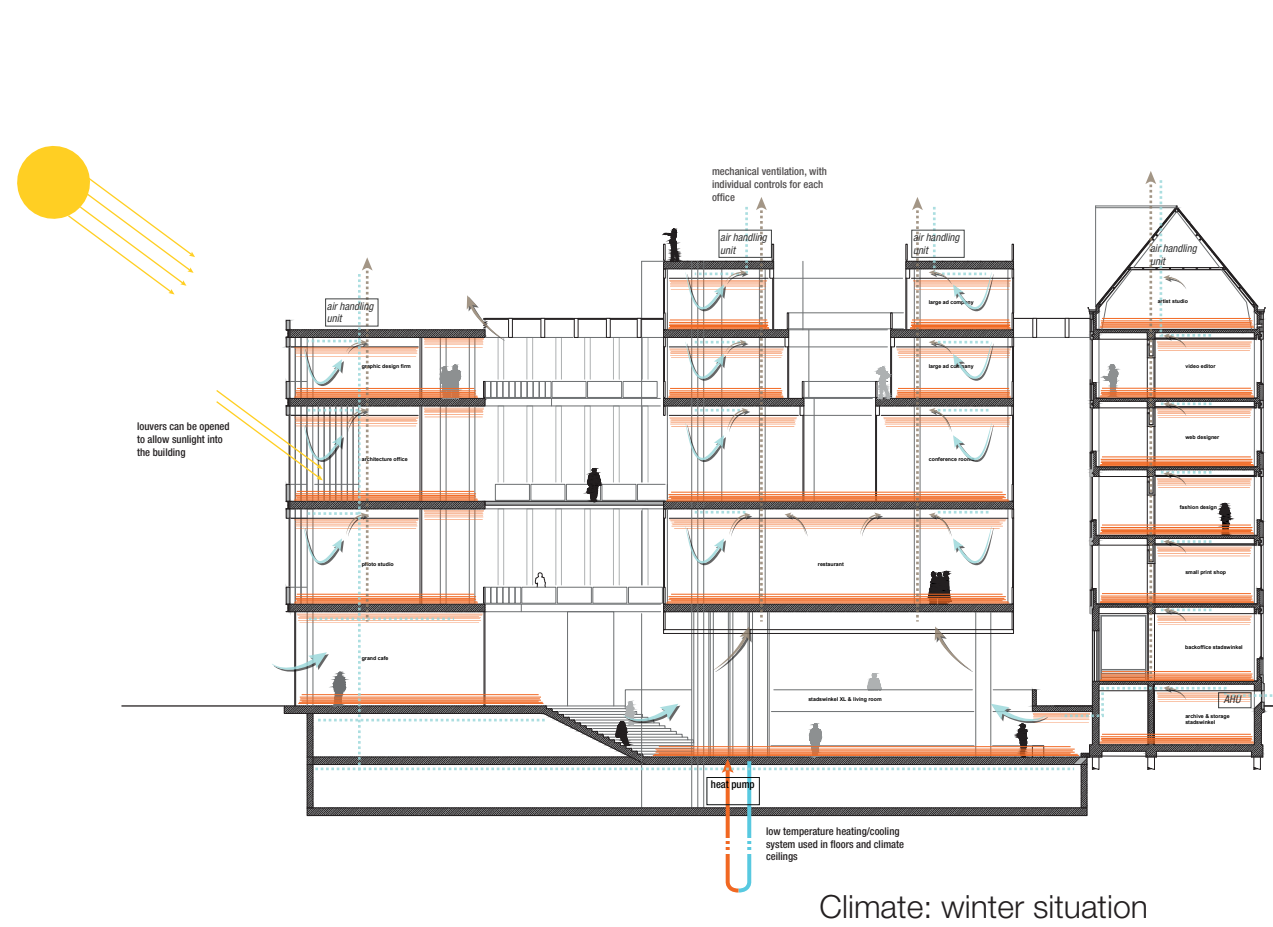
Climate: winter situation
