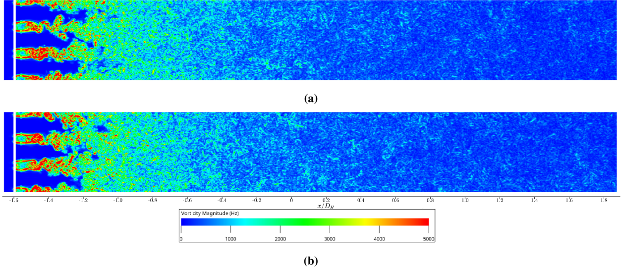
Fig. 8 Vorticity magnitude in the (a) span-wise ( y -aligned) plane and (b) cross-wise ( z -aligned) plane.
