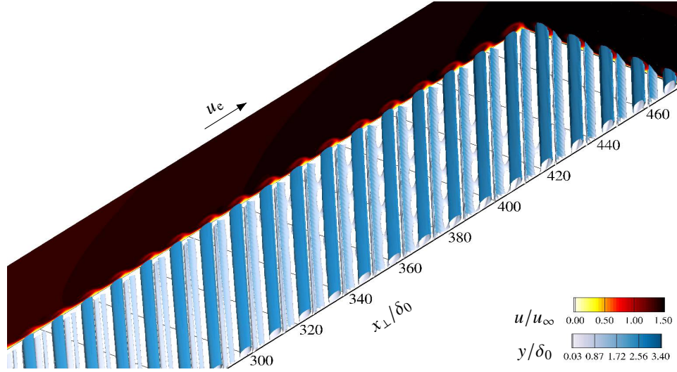
Figure 10 Instantaneous Q -criterion isosurface colored by wall distance and y - z_{||} , x_{\perp} - y planes of instantaneous chordwise velocity. The DNS data are duplicated 4 times in z_{||} in a periodic manner for illustration purposes.
