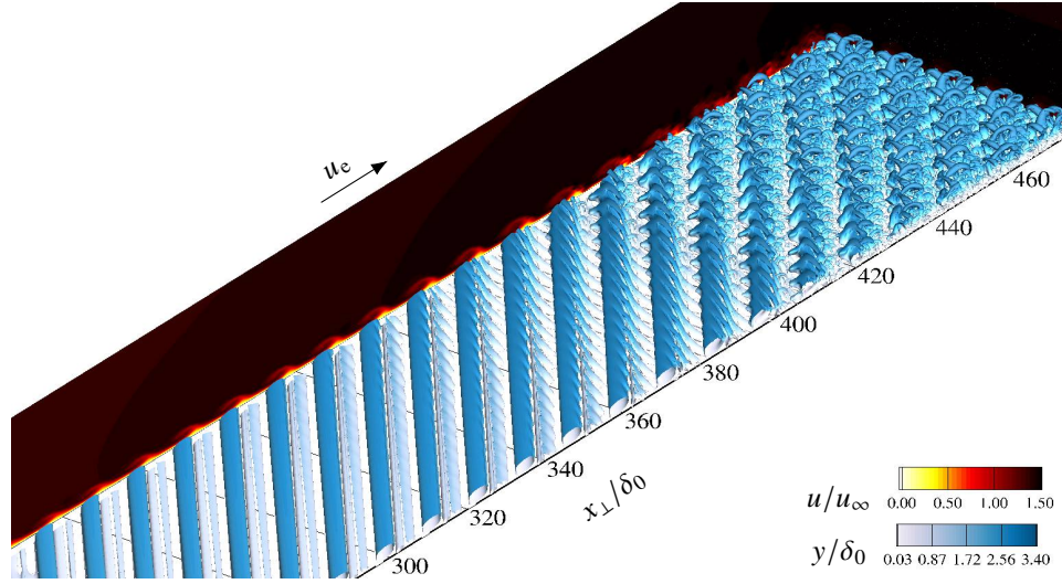
Figure 14 Instantaneous Q -criterion isosurfaces colored by wall distance and y - z_{||} , x_{\perp} - y planes of instantaneous chordwise velocity. The DNS data are duplicated 4 times in z_{||} in a periodic manner for illustration purposes.
