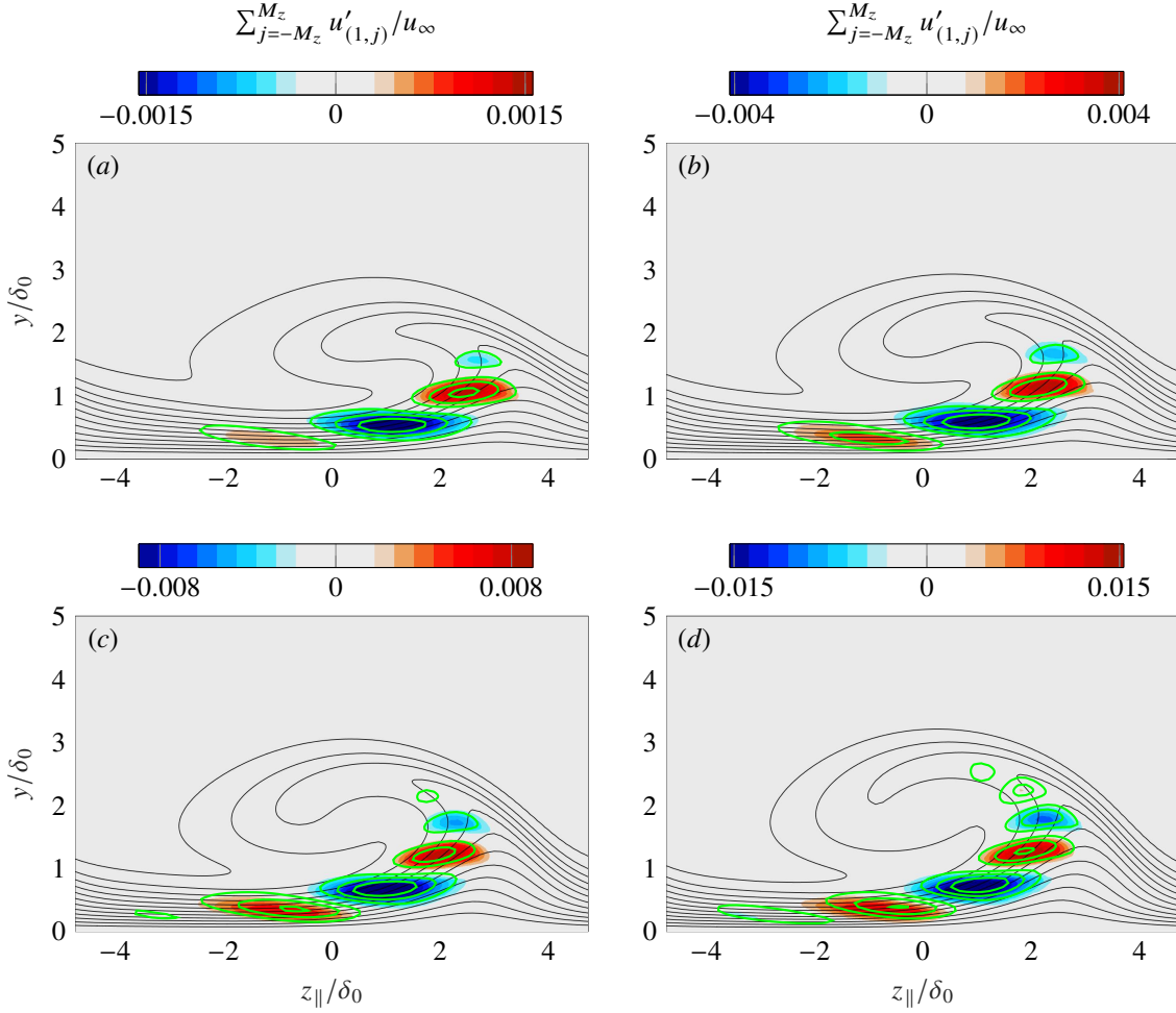
Figure 7 Organization of the unsteady perturbation field \sum_{j=-M_z}^{M_z} u'_{(1,j)}/u_\infty from DNS (color map) and BiGlobal (solid green) at x_\perp/\delta_0 = 316 (a), 341 (b), 365 (c), 390 (d). Isolines of distorted base flow (solid black).
