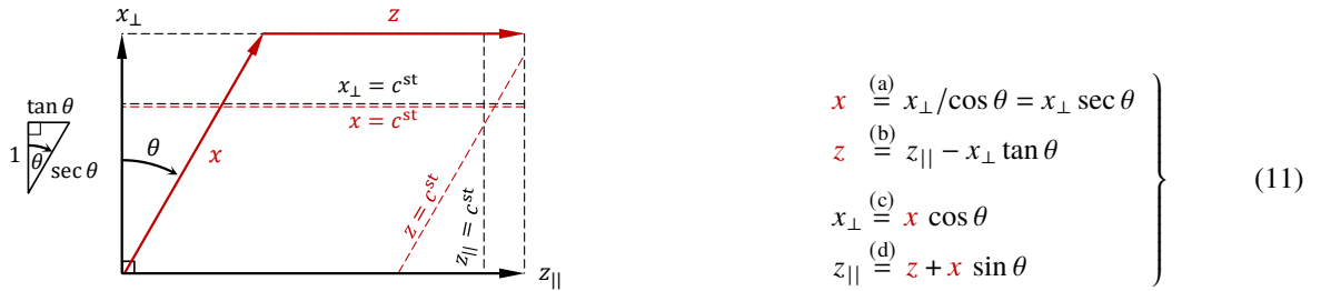
Figure 16 Coordinate systems and transformations.
