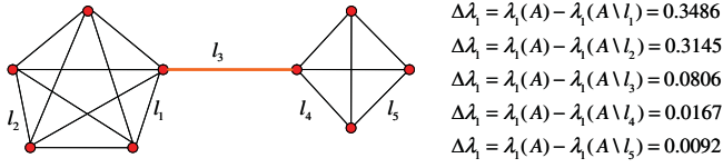
FIG. 6. (Color online) All possible \Delta\lambda_1 are computed when one link is removed.
