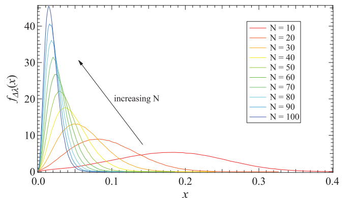
FIG. 11. (Color online) The probability density function of \Delta\lambda_1 for ER random graphs of several sizes N .
