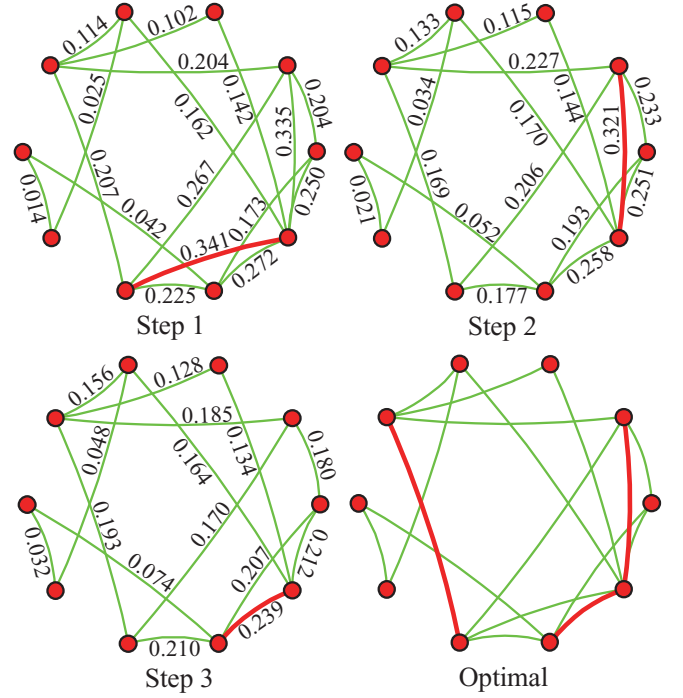
FIG. 3. (Color online) An example of a graph with N = 10 nodes, where two links in the greedy approach appear in the optimal set of links.
