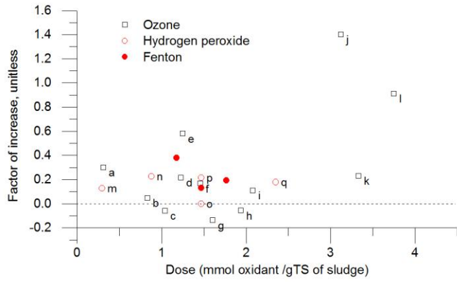
Fig C.1 Effect of oxidant doses in the biogas production. Letters refer to entries in Table 12.
