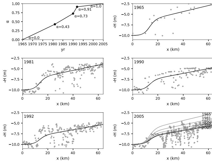
Figure 2. Evolution of the bed profile in the Ems, with in the top-left panel, the development of the bed profile parameter \alpha (equation (1)) over time, obtained by fitting to observed depths in 1965, 1981, 1990, 1992, and 2005 (De Jonge et al., 2014). The other panels show the resulting smooth fitted depth profiles (solid lines) in these years, together with observed thalweg depth (dots). The bottom-right panel for 2005 additionally shows the smooth fitted profiles of the other years for comparison.
