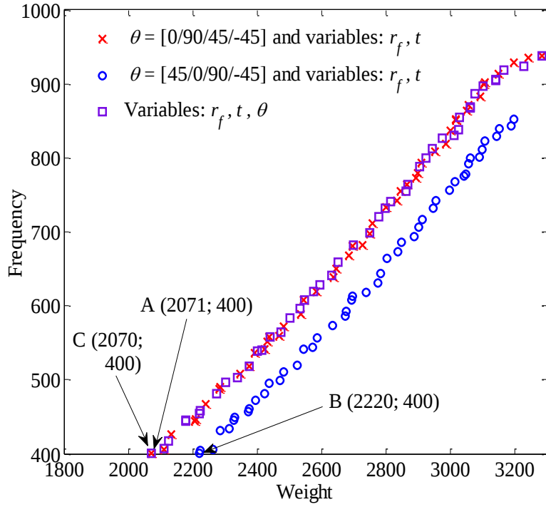
Figure 12. Pareto-optimal solutions of fixed-free beam for model 3 and model 2.
