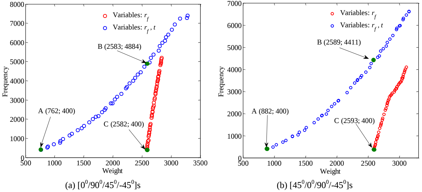
Figure 10. Pareto-optimal solutions of pinned-pinned beam for model 2 and model 1.
