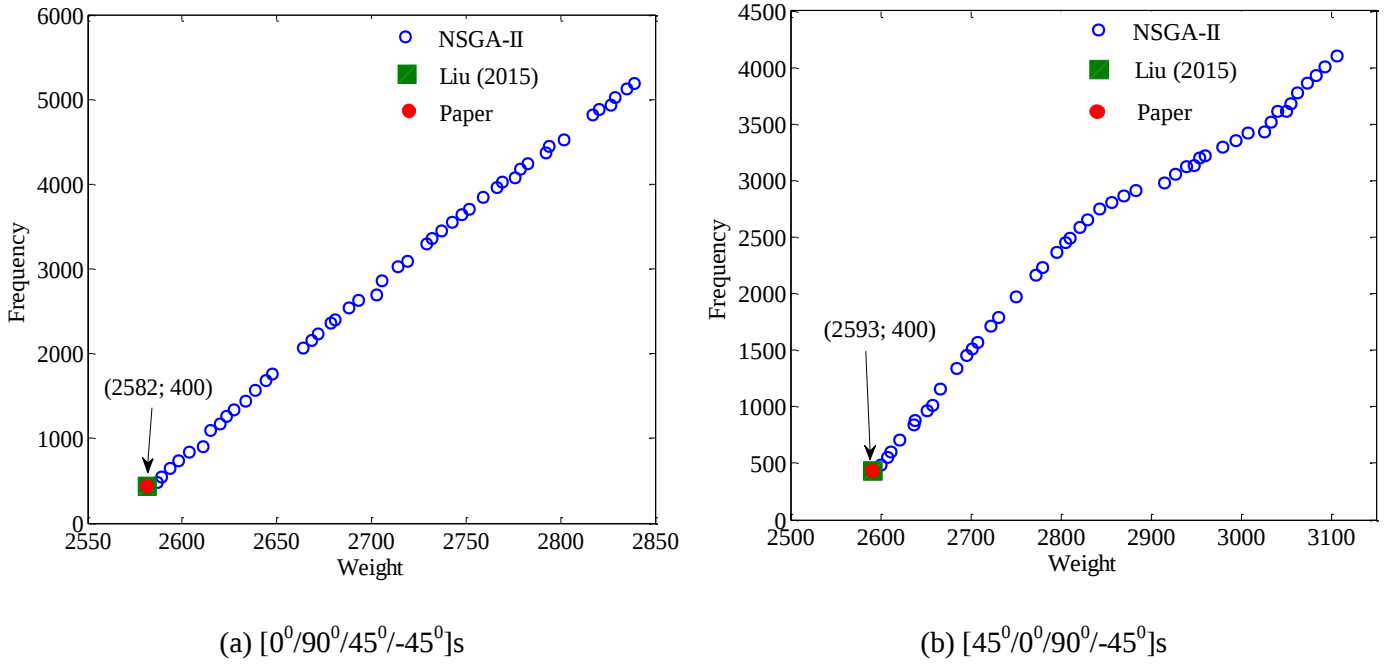
Figure 6. Pareto-optimal solutions of pinned- pinned beam for model 1.
