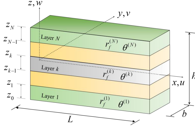
Figure 1. A laminated composite beam.
