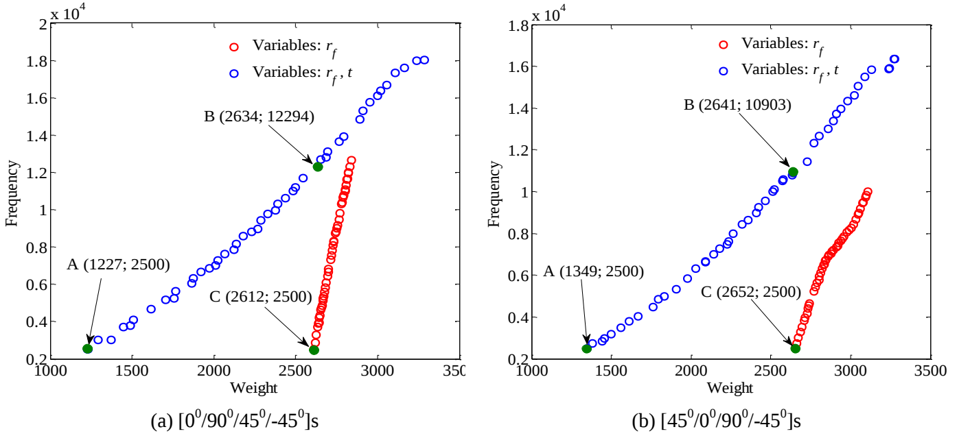
Figure 9. Pareto-optimal solutions of fixed-pinned beam for model 2 and model 1.
