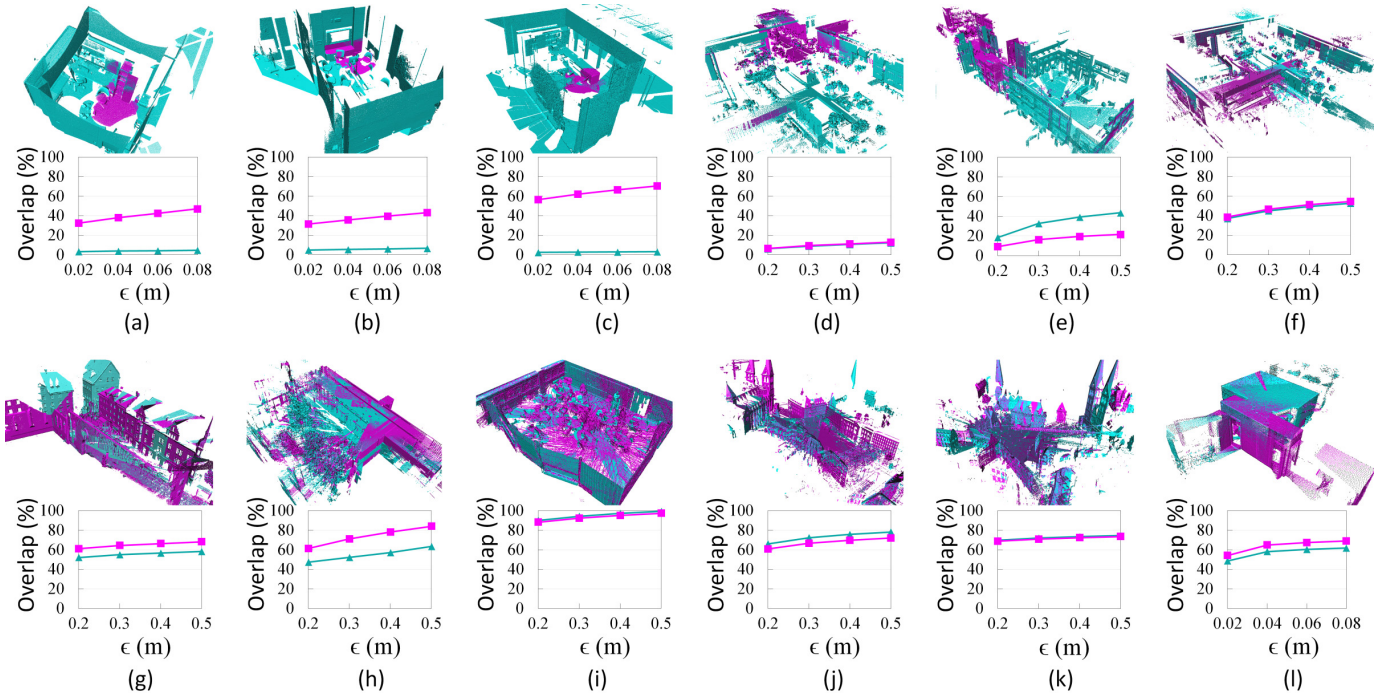
Fig. 5. Overlap of point cloud pairs. (Top Row) Scan pairs from RESSO. (Bottom Row) Scan pairs from existing data sets, i.e., (g) ETH [50], (h) DS2-L [13], (i) TLS-ZEB [14], (j) and (k) Robotic 3-D scan repository [5], and (l) DS1-H [6]. The corresponding \epsilon -overlap curve is shown below each scan pair.
