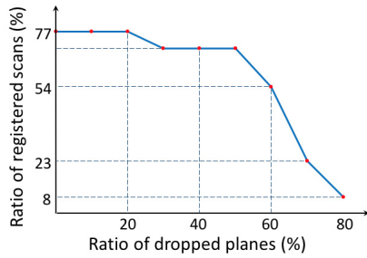
Fig. 10. Registration by gradually dropping planes on the scene shown in Fig. 6(a). Planes with smaller numbers of points are dropped first.
