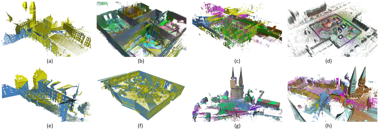
Fig. 8. Registration results of our method on various data sets. (a) Bremen [52]. (b) DS1-H [6]. (c) DS2-L [13]. (d) DS3-V [13]. (e) ETH [50]. (f) TLS-ZEB [14]. (g) and (h) Robotic 3-D scan repository [5]. The ceilings in (b), (c), and (f) have been removed to better reveal the building interiors.
