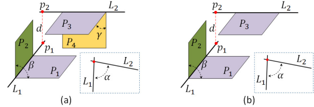
Fig. 2. Structure-level descriptor. (a) Descriptor defined on two pairs of planes. Line L_1 is the intersection of planes P_1 and P_2 ; L_2 is the intersection of planes P_3 and P_4 . (b) Descriptor defined on a line segment L_2 and two planes P_1 and P_2 .
