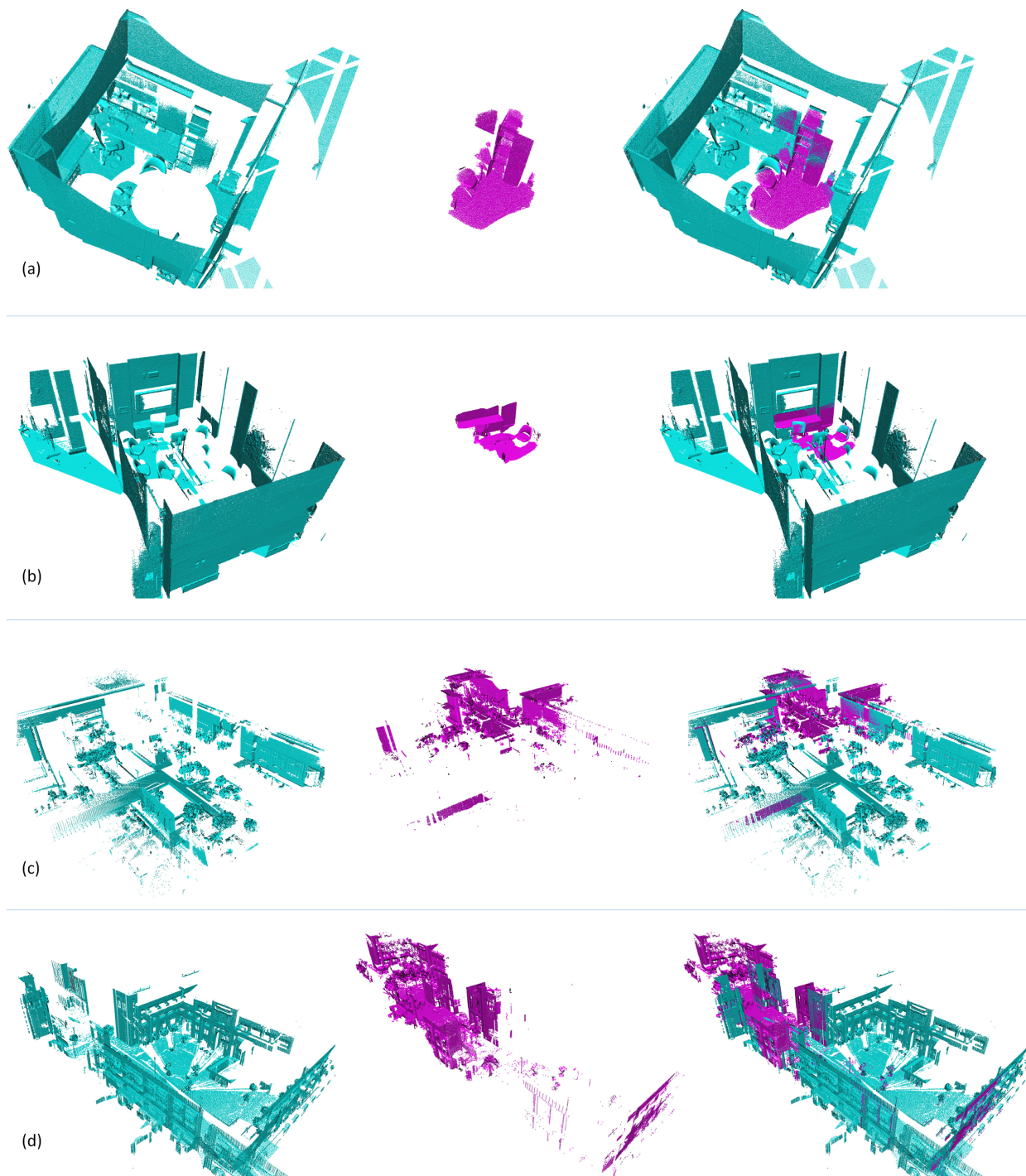
Fig. 9. Pairs of point clouds registered by our method, intended to reveal the overlaps between scans. (First Two Columns) Input scan pairs. (Right Column) Registration results.
